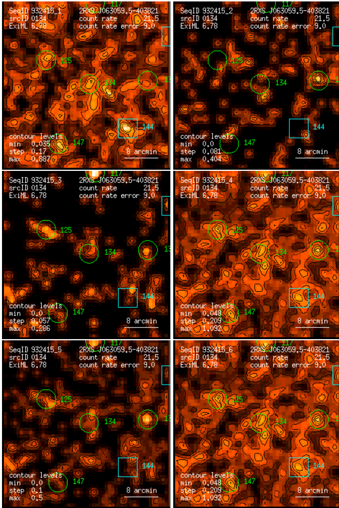
Figure 134: RASS 932415: detection 0134: band rate images, Gaussian filter: (1) PSPC channels 11 – 41, (2) 52 – 90, (3) 91 – 201, (4) 11 – 235, (5) 52 – 201, (6) 11 – 201. Broad band rates in counts/ks. Band rate contour levels in counts/ks/arcmin 2 .
