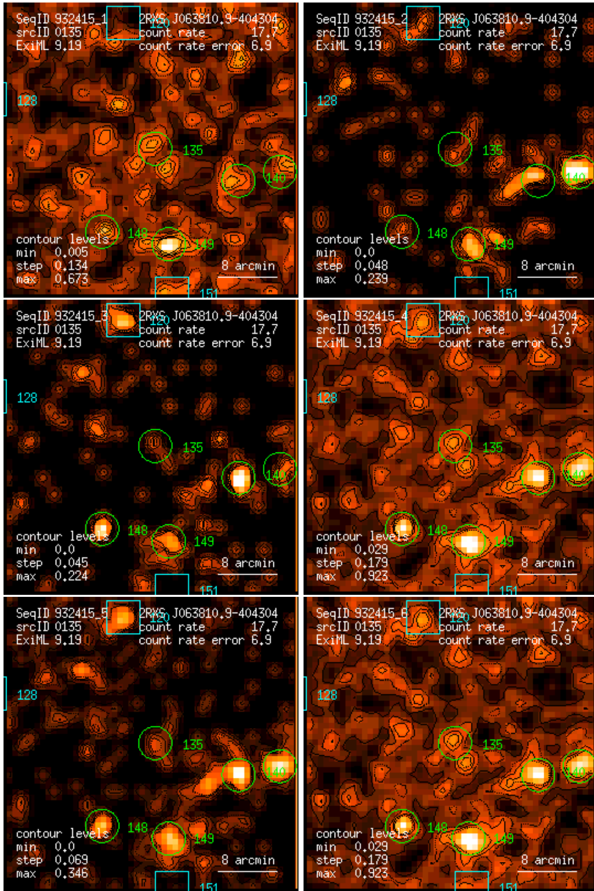
Figure 135: RASS 932415: detection 0135: band rate images, Gaussian filter: (1) PSPC channels 11 – 41, (2) 52 – 90, (3) 91 – 201, (4) 11 – 235, (5) 52 – 201, (6) 11 – 201. Broad band rates in counts/ks. Band rate contour levels in counts/ks/arcmin 2 .
