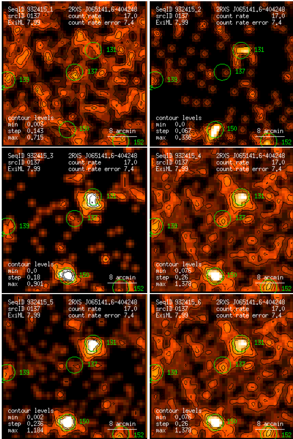
Figure 137: RASS 932415: detection 0137: band rate images, Gaussian filter: (1) PSPC channels 11 – 41, (2) 52 – 90, (3) 91 – 201, (4) 11 – 235, (5) 52 – 201, (6) 11 – 201. Broad band rates in counts/ks. Band rate contour levels in counts/ks/arcmin 2 .
