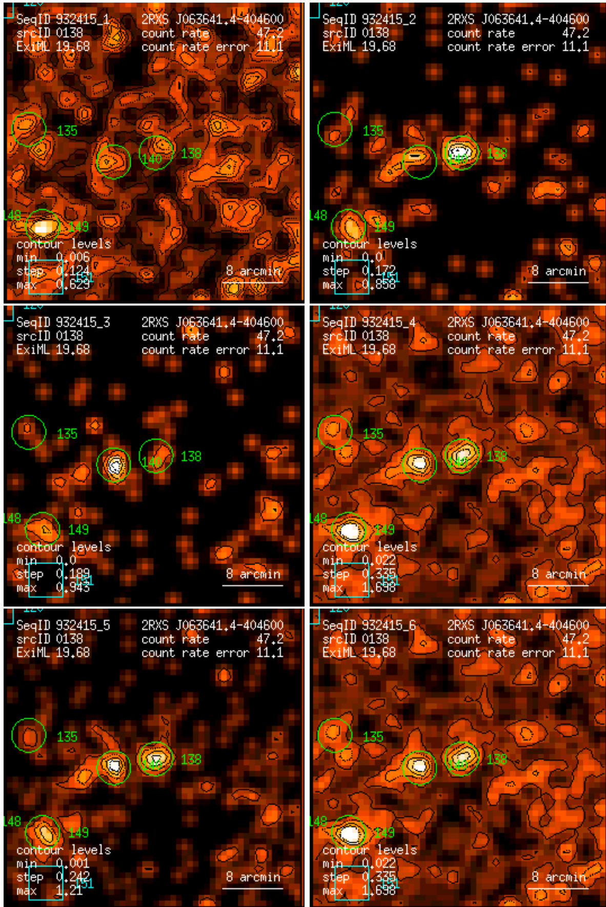
Figure 138: RASS 932415: detection 0138: band rate images, Gaussian filter: (1) PSPC channels 11 – 41, (2) 52 – 90, (3) 91 – 201, (4) 11 – 235, (5) 52 – 201, (6) 11 – 201. Broad band rates in counts/ks. Band rate contour levels in counts/ks/arcmin 2 .
