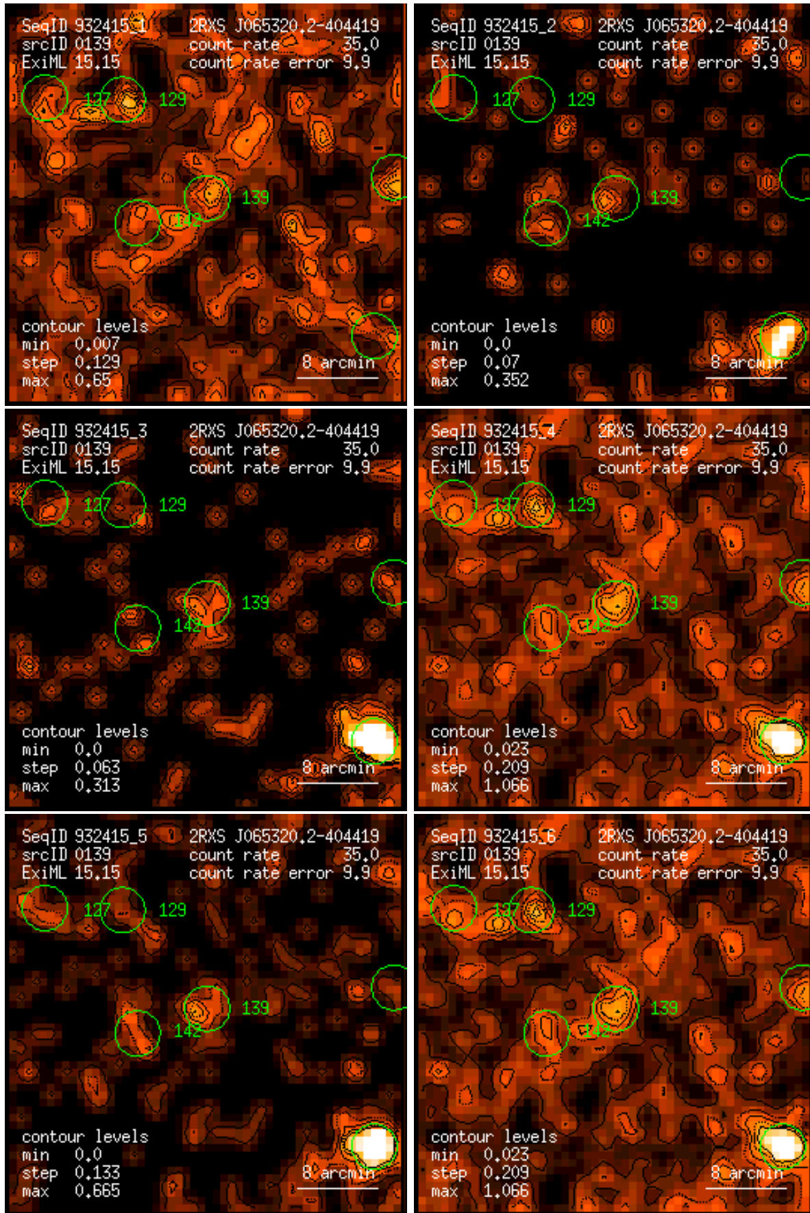
Figure 139: RASS 932415: detection 0139: band rate images, Gaussian filter: (1) PSPC channels 11 – 41, (2) 52 – 90, (3) 91 – 201, (4) 11 – 235, (5) 52 – 201, (6) 11 – 201. Broad band rates in counts/ks. Band rate contour levels in counts/ks/arcmin 2 .
