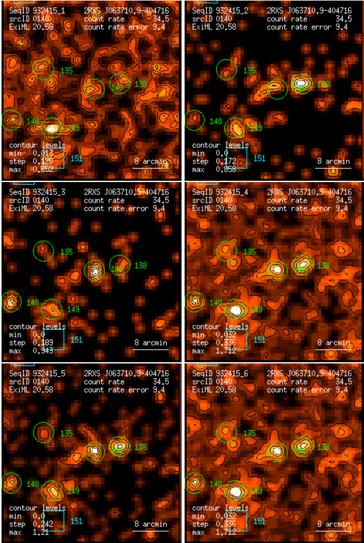
Figure 140: RASS 932415: detection 0140: band rate images, Gaussian filter: (1) PSPC channels 11 – 41, (2) 52 – 90, (3) 91 – 201, (4) 11 – 235, (5) 52 – 201, (6) 11 – 201. Broad band rates in counts/ks. Band rate contour levels in counts/ks/arcmin 2 .
