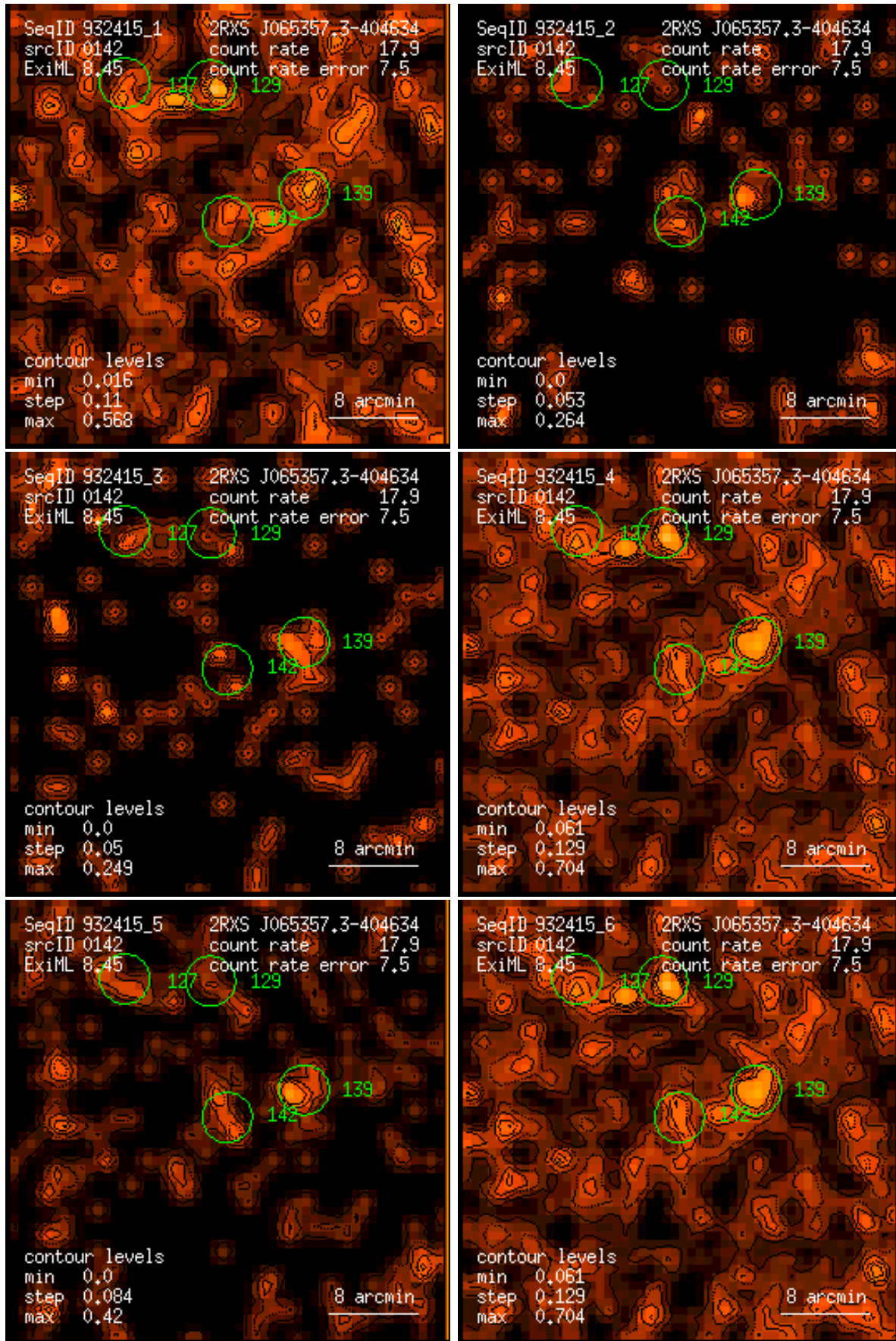
Figure 142: RASS 932415: detection 0142: band rate images, Gaussian filter: (1) PSPC channels 11 – 41, (2) 52 – 90, (3) 91 – 201, (4) 11 – 235, (5) 52 – 201, (6) 11 – 201. Broad band rates in counts/ks. Band rate contour levels in counts/ks/arcmin 2 .
