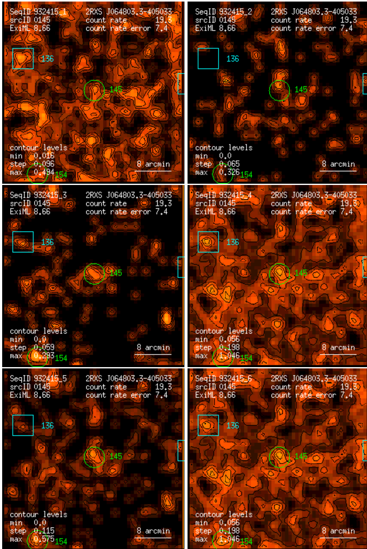
Figure 145: RASS 932415: detection 0145: band rate images, Gaussian filter: (1) PSPC channels 11 – 41, (2) 52 – 90, (3) 91 – 201, (4) 11 – 235, (5) 52 – 201, (6) 11 – 201. Broad band rates in counts/ks. Band rate contour levels in counts/ks/arcmin 2 .
