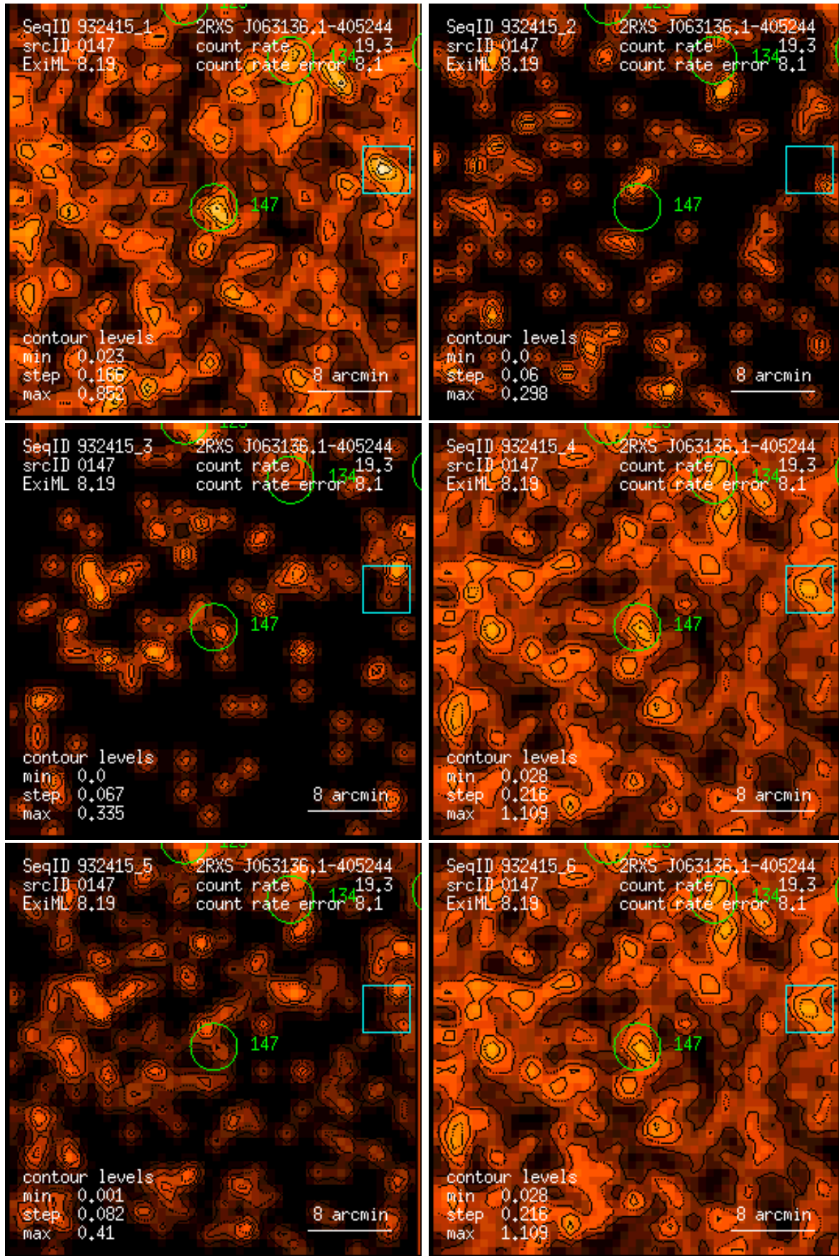
Figure 147: RASS 932415: detection 0147: band rate images, Gaussian filter: (1) PSPC channels 11 – 41, (2) 52 – 90, (3) 91 – 201, (4) 11 – 235, (5) 52 – 201, (6) 11 – 201. Broad band rates in counts/ks. Band rate contour levels in counts/ks/arcmin 2 .
