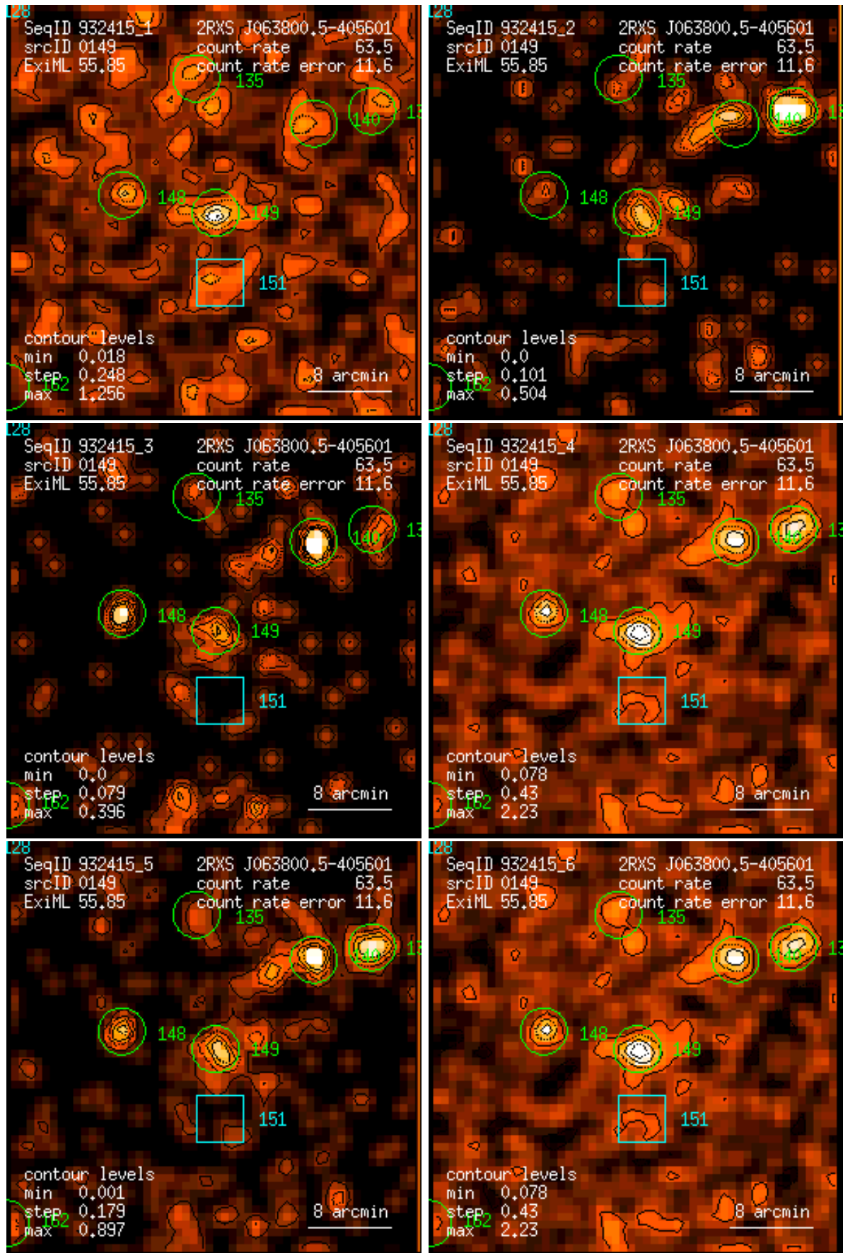
Figure 149: RASS 932415: detection 0149: band rate images, Gaussian filter: (1) PSPC channels 11 – 41, (2) 52 – 90, (3) 91 – 201, (4) 11 – 235, (5) 52 – 201, (6) 11 – 201. Broad band rates in counts/ks. Band rate contour levels in counts/ks/arcmin 2 .
