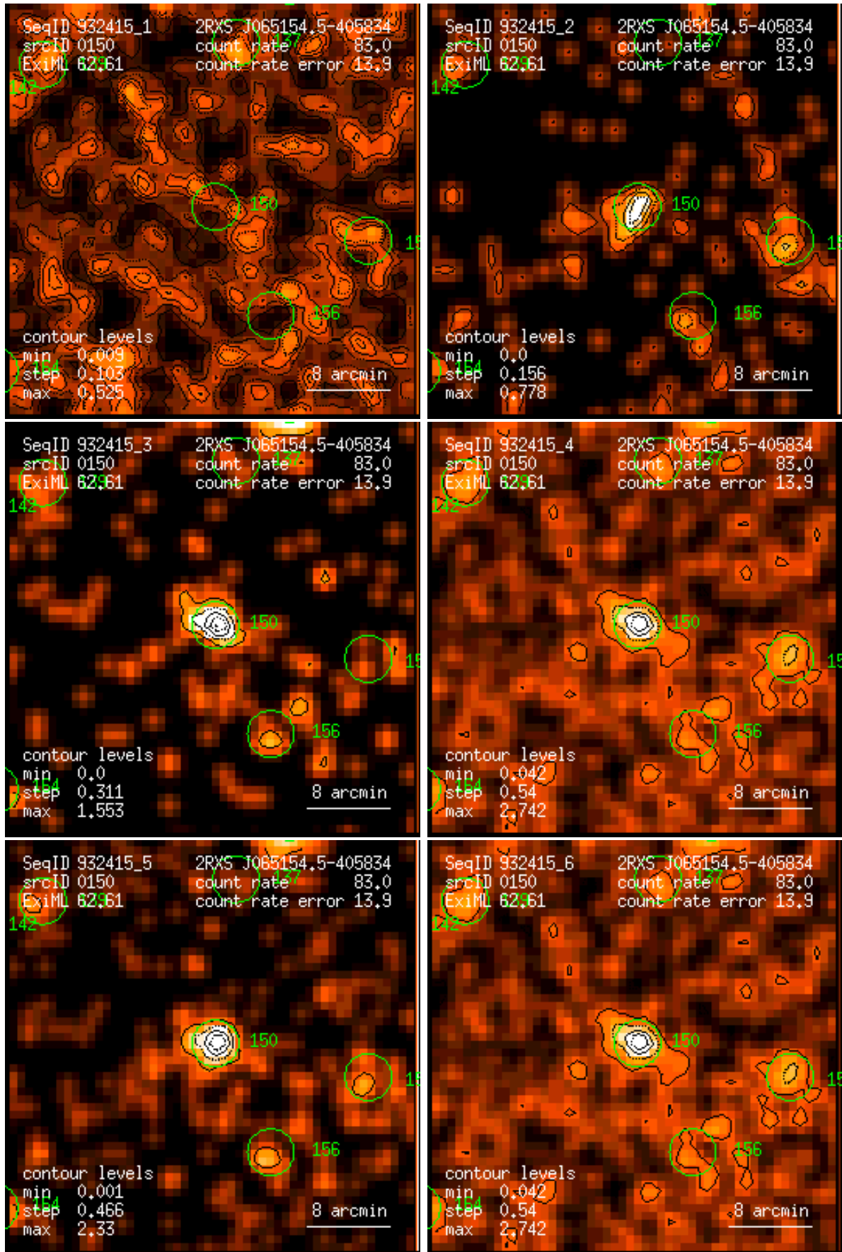
Figure 150: RASS 932415: detection 0150: band rate images, Gaussian filter: (1) PSPC channels 11 – 41, (2) 52 – 90, (3) 91 – 201, (4) 11 – 235, (5) 52 – 201, (6) 11 – 201. Broad band rates in counts/ks. Band rate contour levels in counts/ks/arcmin 2 .
