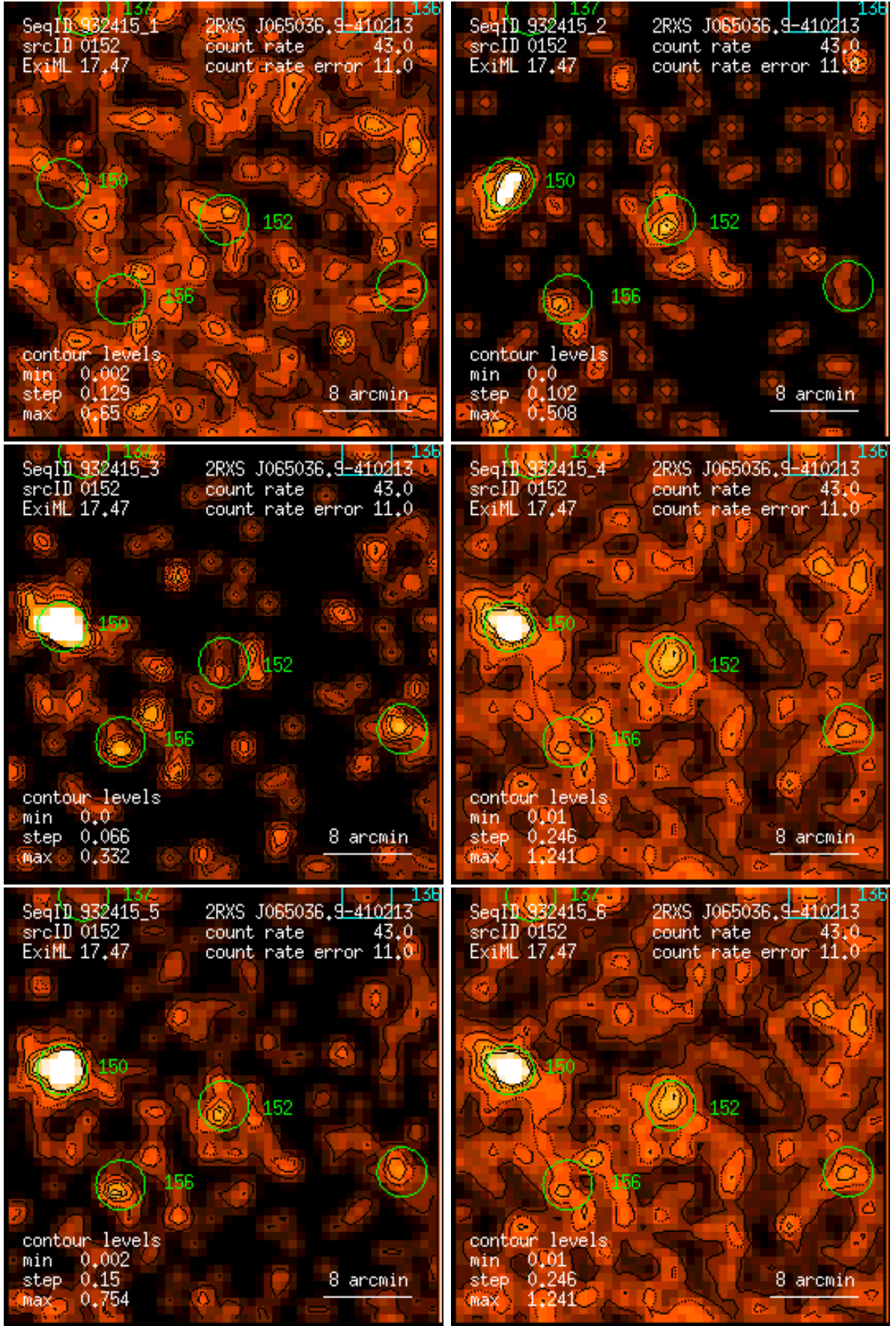
Figure 152: RASS 932415: detection 0152: band rate images, Gaussian filter: (1) PSPC channels 11 – 41, (2) 52 – 90, (3) 91 – 201, (4) 11 – 235, (5) 52 – 201, (6) 11 – 201. Broad band rates in counts/ks. Band rate contour levels in counts/ks/arcmin 2 .
