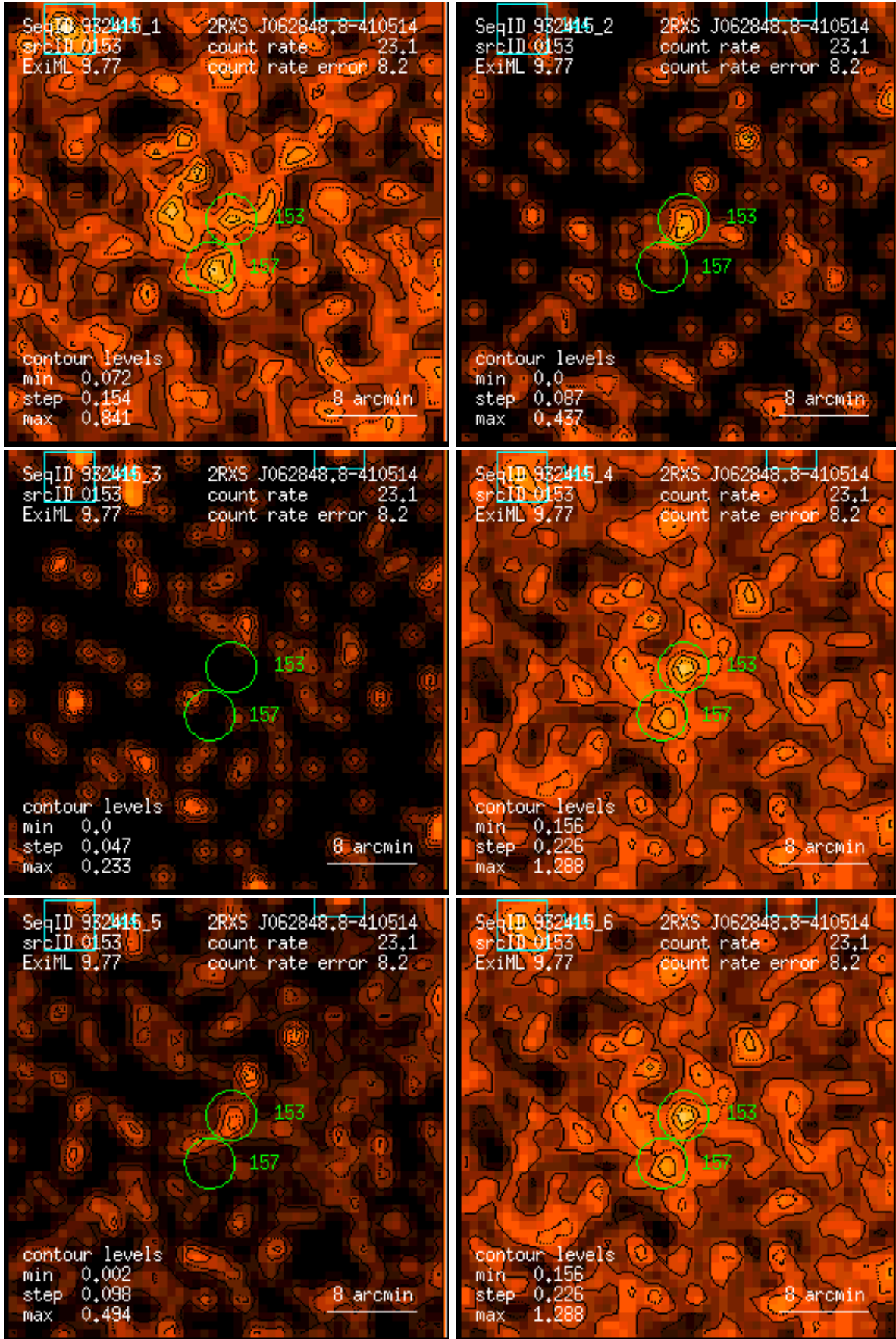
Figure 153: RASS 932415: detection 0153: band rate images, Gaussian filter: (1) PSPC channels 11 – 41, (2) 52 – 90, (3) 91 – 201, (4) 11 – 235, (5) 52 – 201, (6) 11 – 201. Broad band rates in counts/ks. Band rate contour levels in counts/ks/arcmin 2 .
