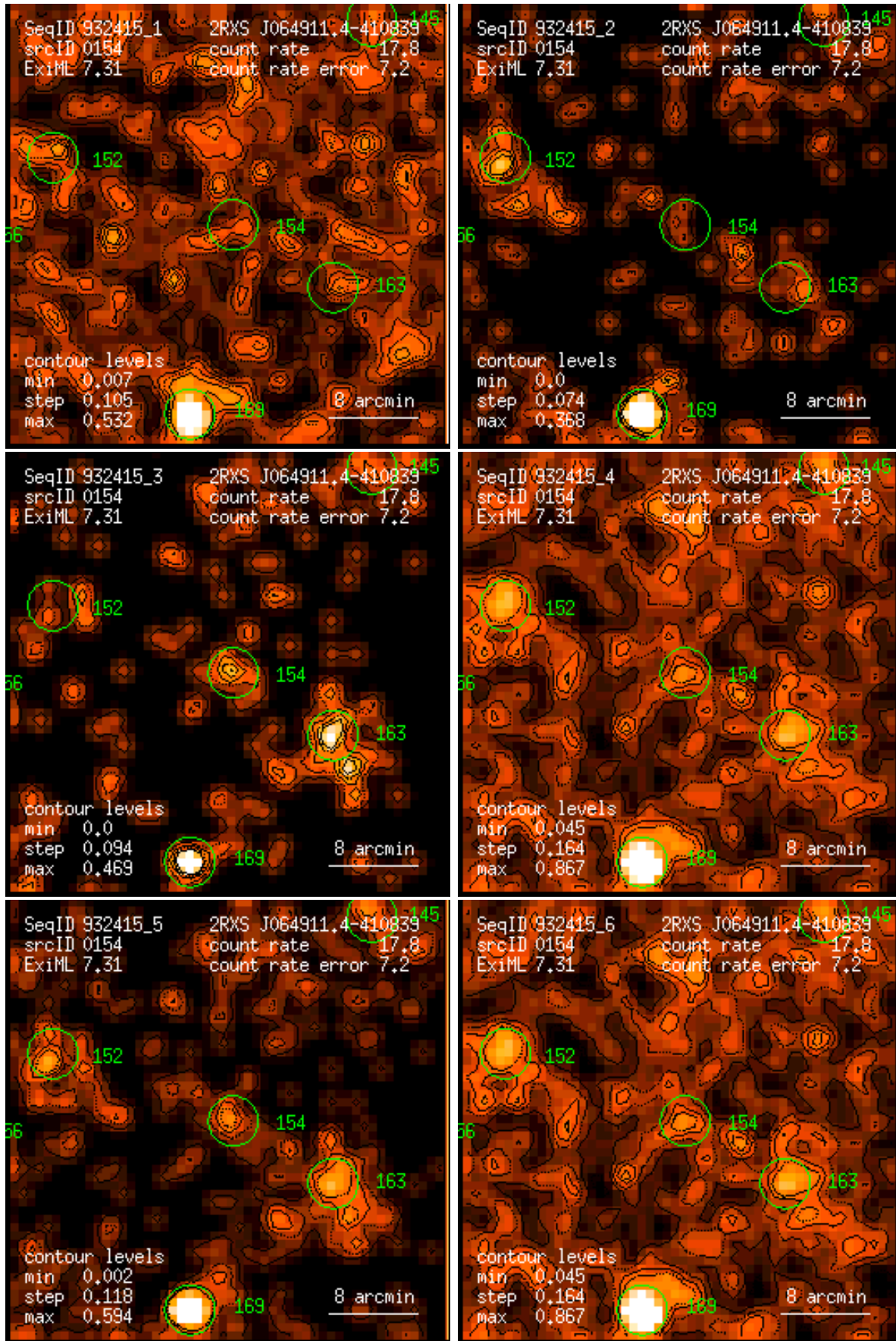
Figure 154: RASS 932415: detection 0154: band rate images, Gaussian filter: (1) PSPC channels 11 – 41, (2) 52 – 90, (3) 91 – 201, (4) 11 – 235, (5) 52 – 201, (6) 11 – 201. Broad band rates in counts/ks. Band rate contour levels in counts/ks/arcmin 2 .
