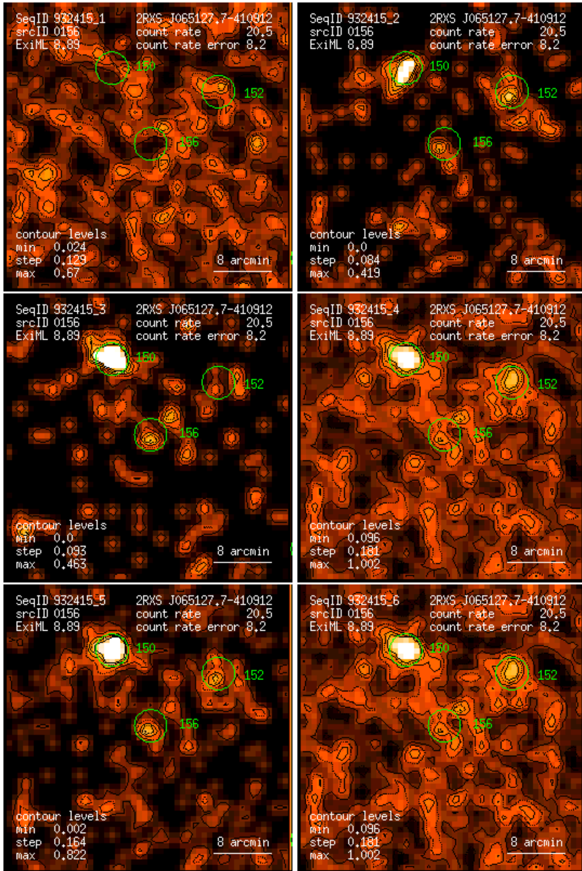
Figure 156: RASS 932415: detection 0156: band rate images, Gaussian filter: (1) PSPC channels 11 – 41, (2) 52 – 90, (3) 91 – 201, (4) 11 – 235, (5) 52 – 201, (6) 11 – 201. Broad band rates in counts/ks. Band rate contour levels in counts/ks/arcmin 2 .
