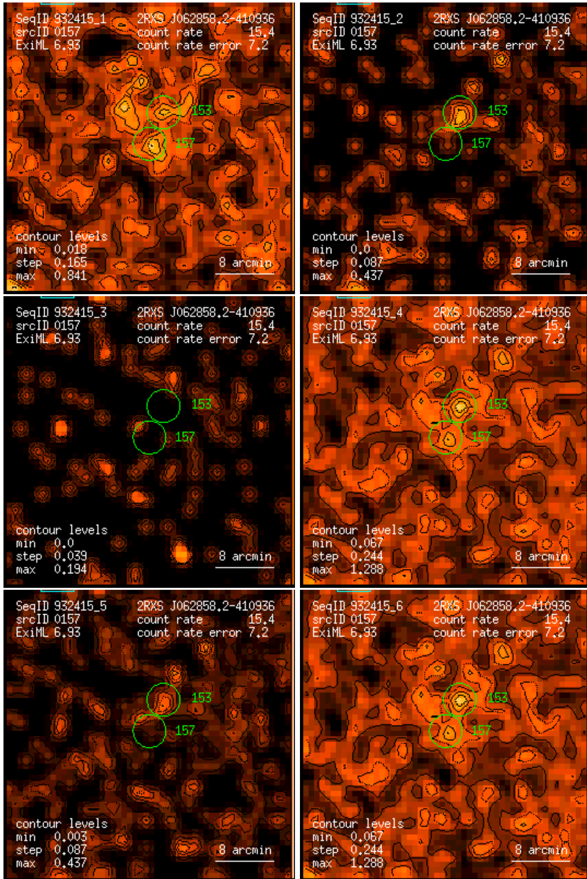
Figure 157: RASS 932415: detection 0157: band rate images, Gaussian filter: (1) PSPC channels 11 – 41, (2) 52 – 90, (3) 91 – 201, (4) 11 – 235, (5) 52 – 201, (6) 11 – 201. Broad band rates in counts/ks. Band rate contour levels in counts/ks/arcmin 2 .
