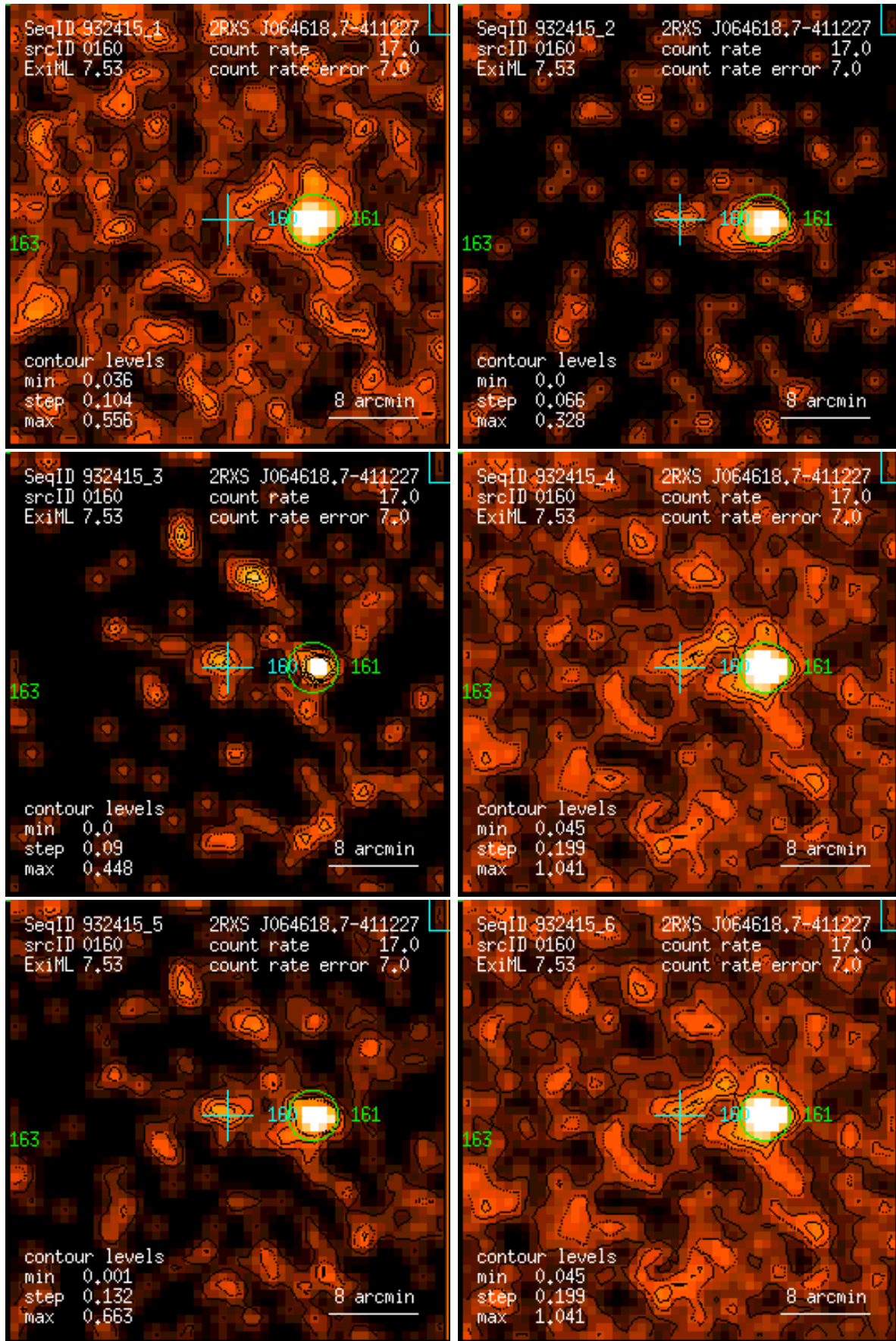
Figure 160: RASS 932415: detection 0160: band rate images, Gaussian filter: (1) PSPC channels 11 – 41, (2) 52 – 90, (3) 91 – 201, (4) 11 – 235, (5) 52 – 201, (6) 11 – 201. Broad band rates in counts/ks. Band rate contour levels in counts/ks/arcmin 2 .
