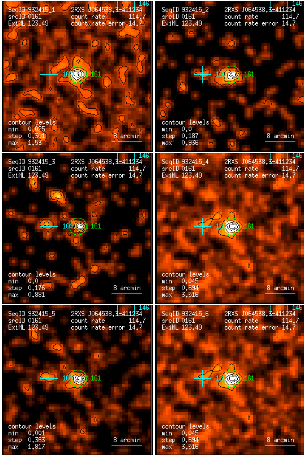
Figure 161: RASS 932415: detection 0161: band rate images, Gaussian filter: (1) PSPC channels 11 – 41, (2) 52 – 90, (3) 91 – 201, (4) 11 – 235, (5) 52 – 201, (6) 11 – 201. Broad band rates in counts/ks. Band rate contour levels in counts/ks/arcmin 2 .
