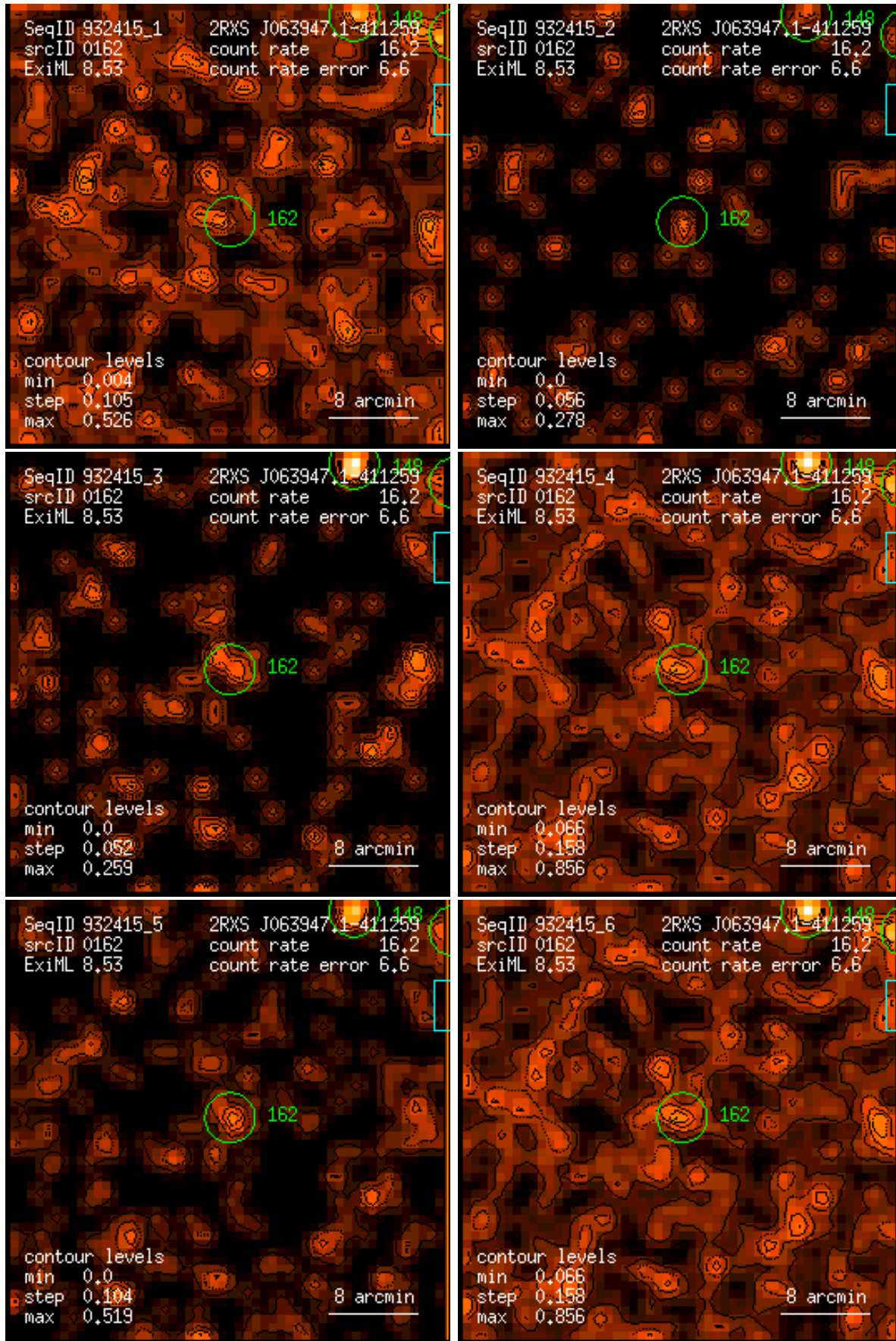
Figure 162: RASS 932415: detection 0162: band rate images, Gaussian filter: (1) PSPC channels 11 – 41, (2) 52 – 90, (3) 91 – 201, (4) 11 – 235, (5) 52 – 201, (6) 11 – 201. Broad band rates in counts/ks. Band rate contour levels in counts/ks/arcmin 2 .
