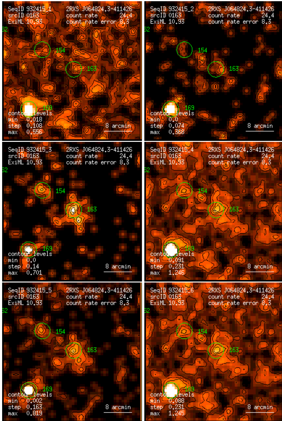
Figure 163: RASS 932415: detection 0163: band rate images, Gaussian filter: (1) PSPC channels 11 – 41, (2) 52 – 90, (3) 91 – 201, (4) 11 – 235, (5) 52 – 201, (6) 11 – 201. Broad band rates in counts/ks. Band rate contour levels in counts/ks/arcmin 2 .
