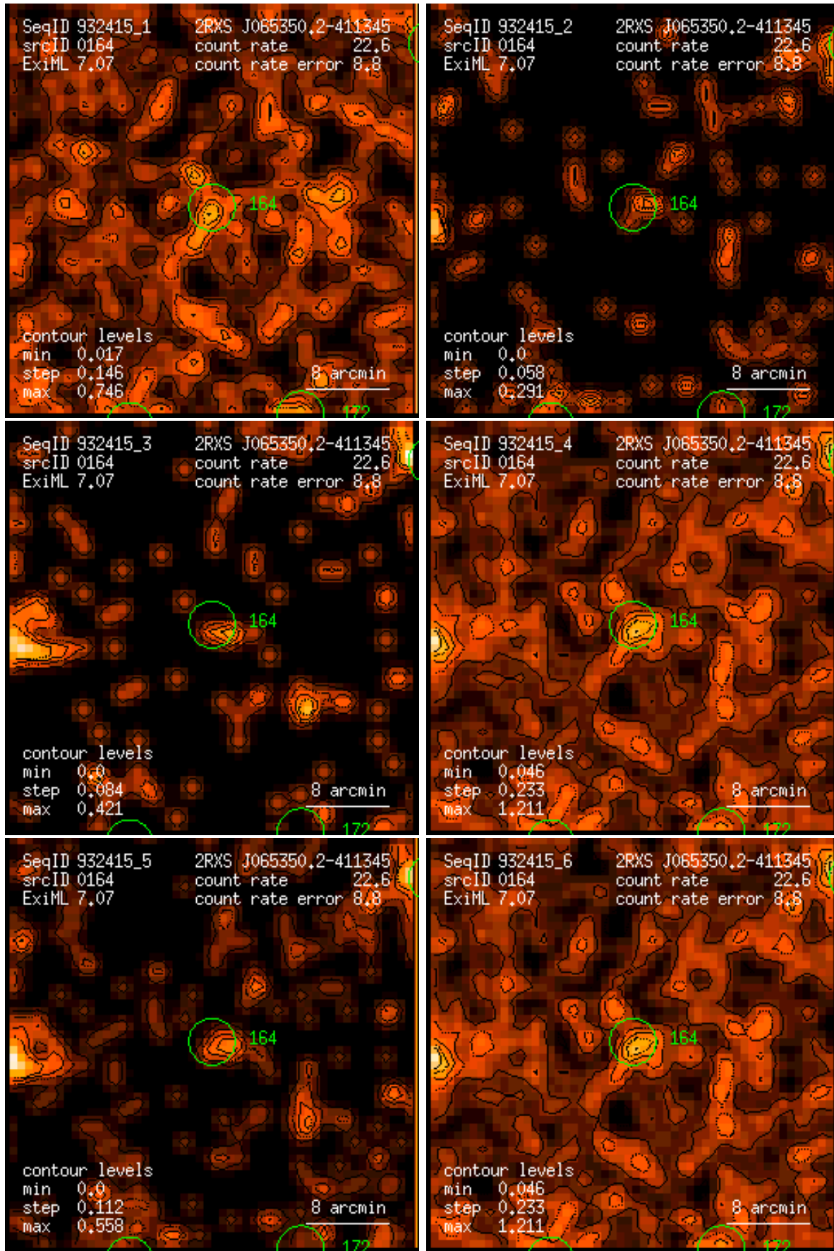
Figure 164: RASS 932415: detection 0164: band rate images, Gaussian filter: (1) PSPC channels 11 – 41, (2) 52 – 90, (3) 91 – 201, (4) 11 – 235, (5) 52 – 201, (6) 11 – 201. Broad band rates in counts/ks. Band rate contour levels in counts/ks/arcmin 2 .
