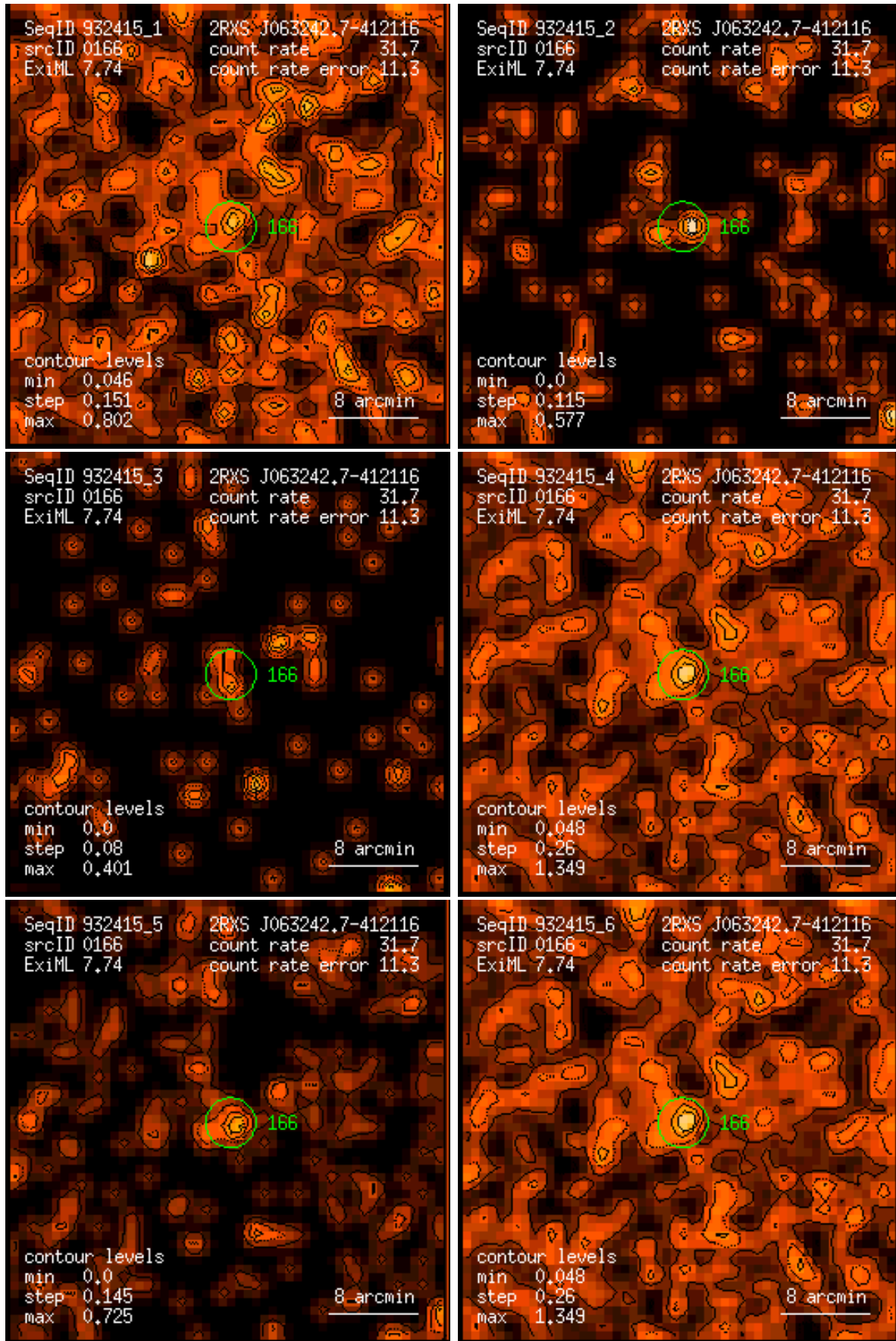
Figure 166: RASS 932415: detection 0166: band rate images, Gaussian filter: (1) PSPC channels 11 – 41, (2) 52 – 90, (3) 91 – 201, (4) 11 – 235, (5) 52 – 201, (6) 11 – 201. Broad band rates in counts/ks. Band rate contour levels in counts/ks/arcmin 2 .
