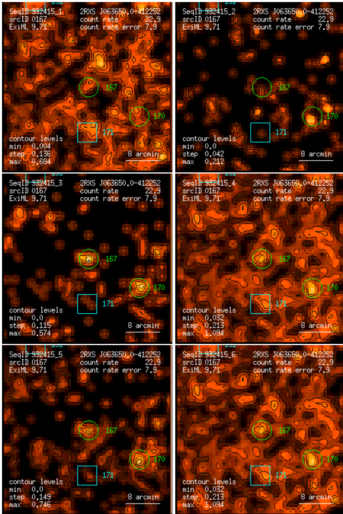
Figure 167: RASS 932415: detection 0167: band rate images, Gaussian filter: (1) PSPC channels 11 – 41, (2) 52 – 90, (3) 91 – 201, (4) 11 – 235, (5) 52 – 201, (6) 11 – 201. Broad band rates in counts/ks. Band rate contour levels in counts/ks/arcmin 2 .
