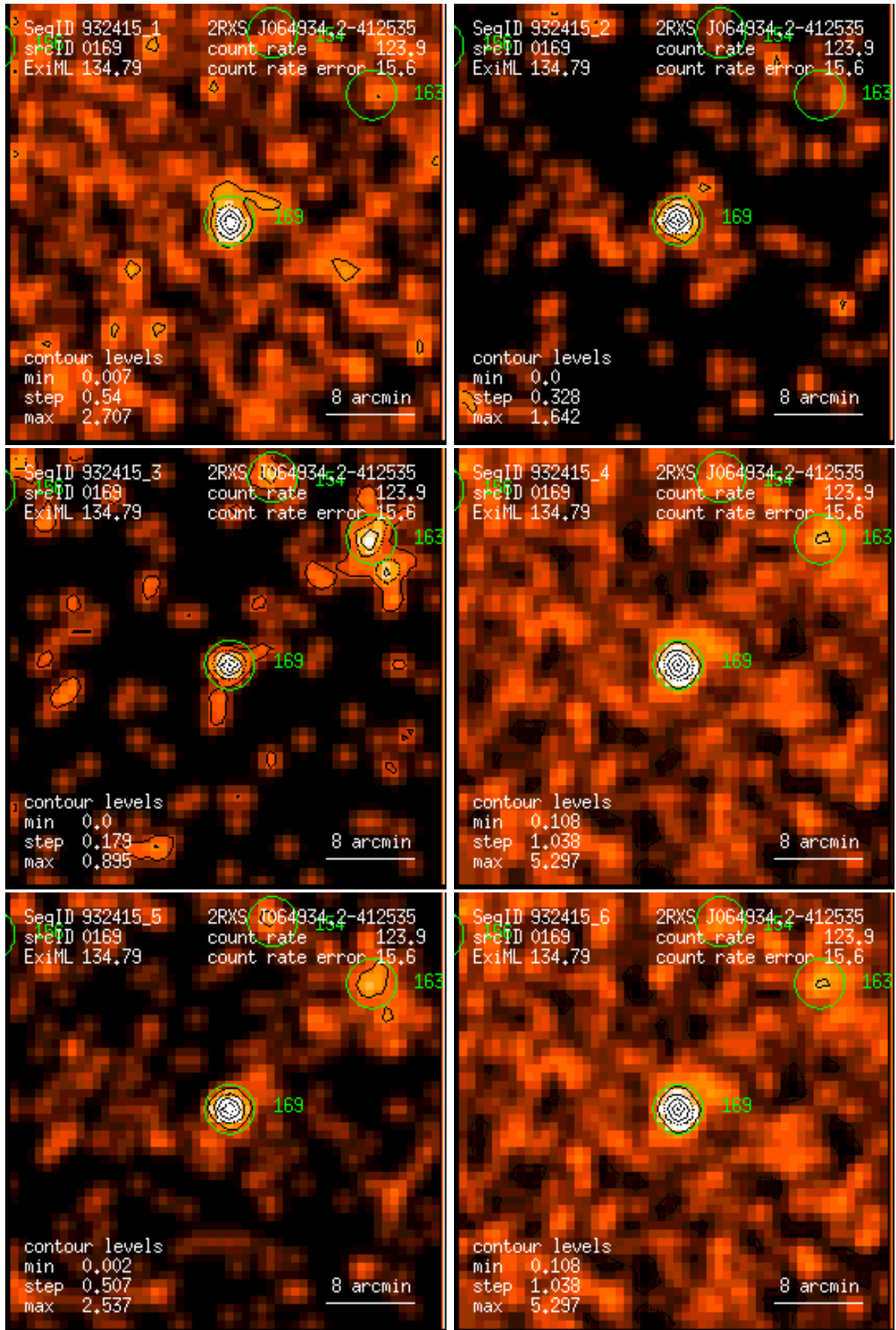
Figure 169: RASS 932415: detection 0169: band rate images, Gaussian filter: (1) PSPC channels 11 – 41, (2) 52 – 90, (3) 91 – 201, (4) 11 – 235, (5) 52 – 201, (6) 11 – 201. Broad band rates in counts/ks. Band rate contour levels in counts/ks/arcmin 2 .
