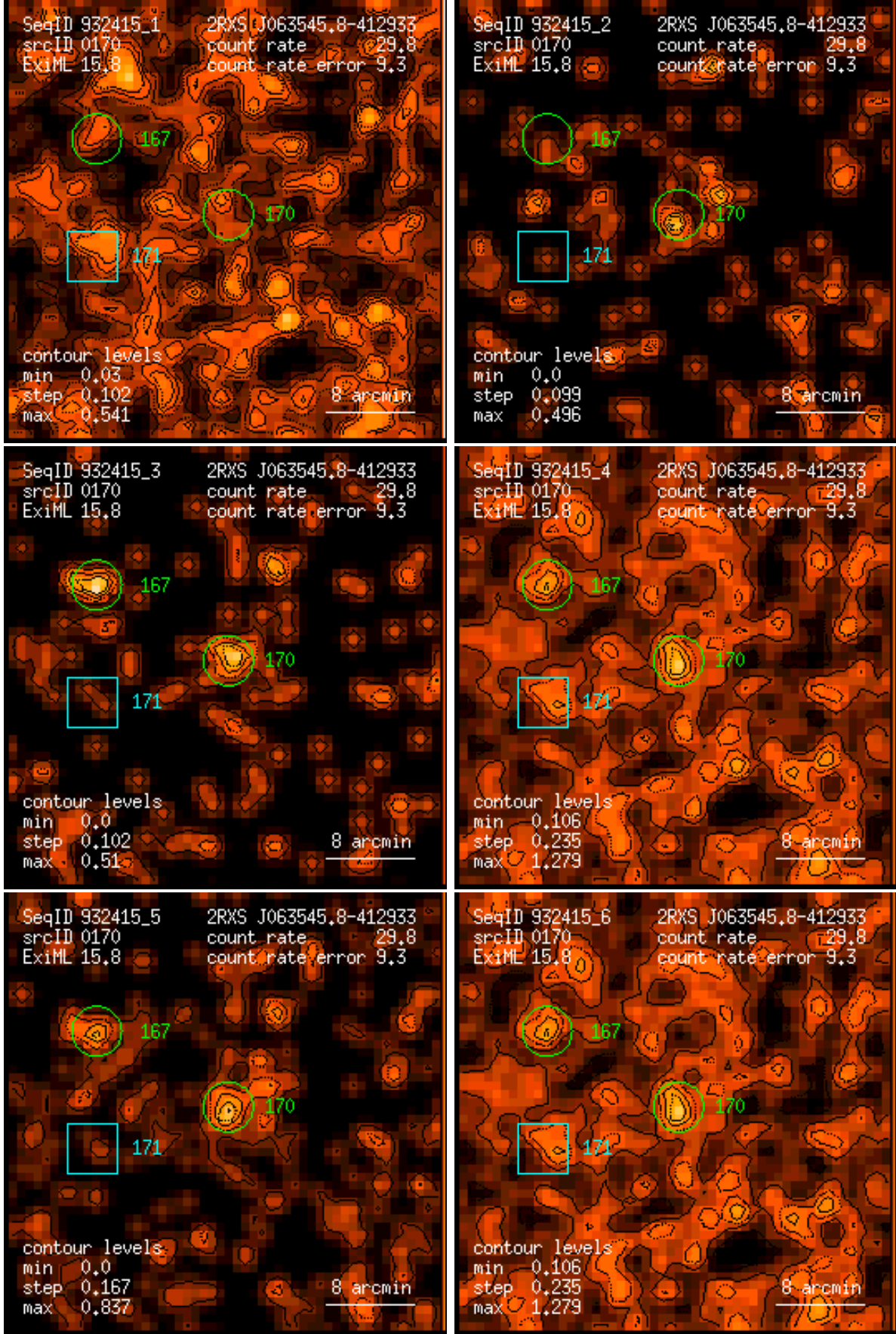
Figure 170: RASS 932415: detection 0170: band rate images, Gaussian filter: (1) PSPC channels 11 – 41, (2) 52 – 90, (3) 91 – 201, (4) 11 – 235, (5) 52 – 201, (6) 11 – 201. Broad band rates in counts/ks. Band rate contour levels in counts/ks/arcmin 2 .
