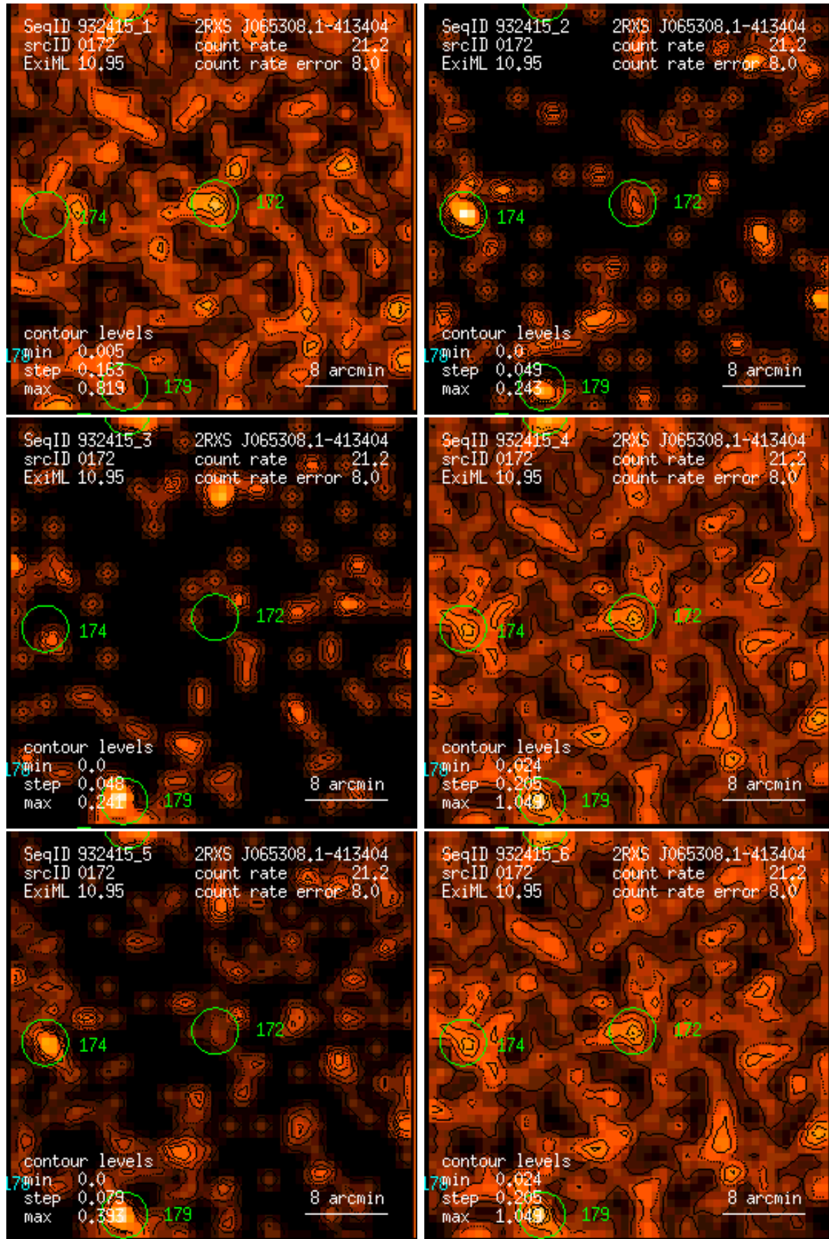
Figure 172: RASS 932415: detection 0172: band rate images, Gaussian filter: (1) PSPC channels 11 – 41, (2) 52 – 90, (3) 91 – 201, (4) 11 – 235, (5) 52 – 201, (6) 11 – 201. Broad band rates in counts/ks. Band rate contour levels in counts/ks/arcmin 2 .
