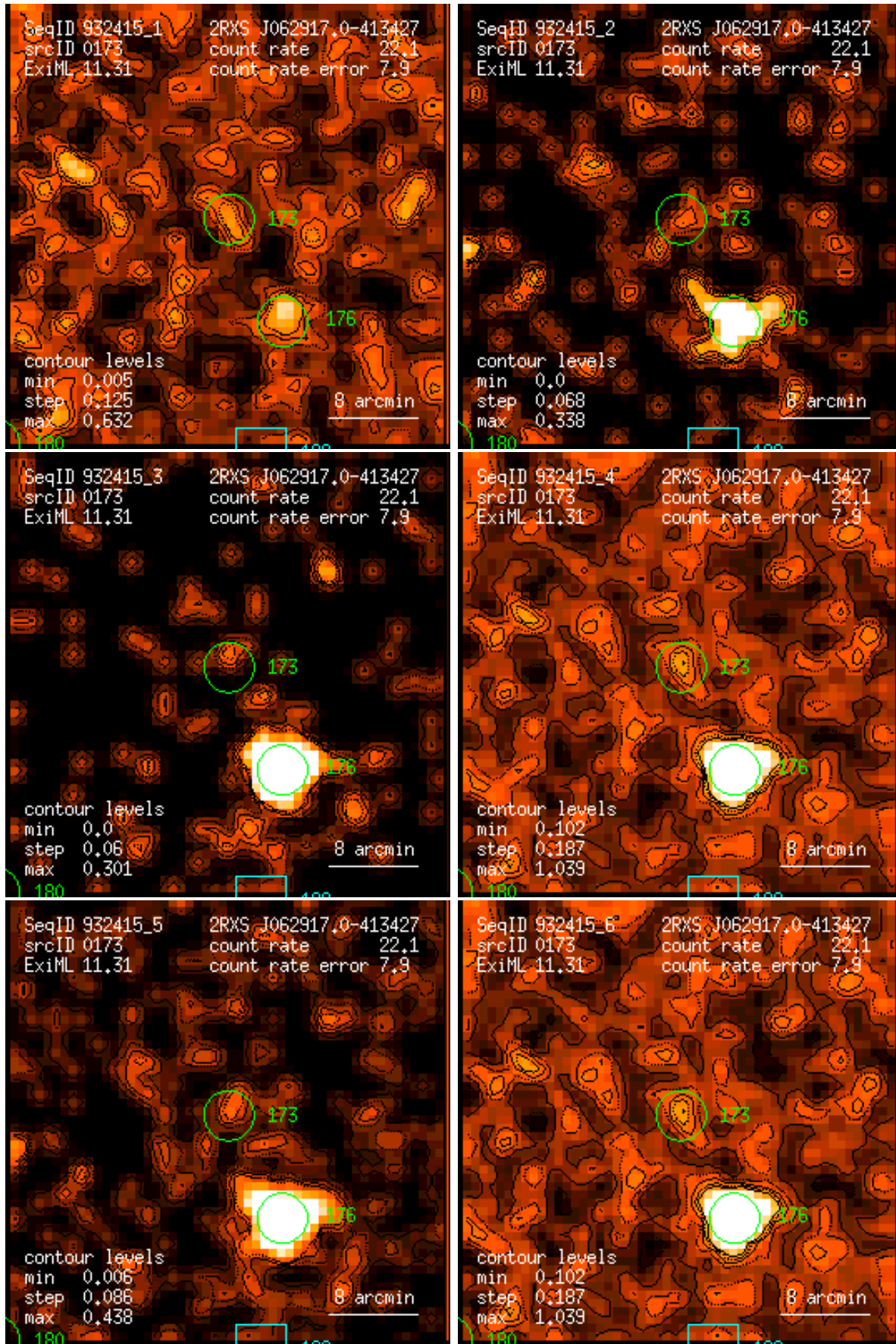
Figure 173: RASS 932415: detection 0173: band rate images, Gaussian filter: (1) PSPC channels 11 – 41, (2) 52 – 90, (3) 91 – 201, (4) 11 – 235, (5) 52 – 201, (6) 11 – 201. Broad band rates in counts/ks. Band rate contour levels in counts/ks/arcmin 2 .
