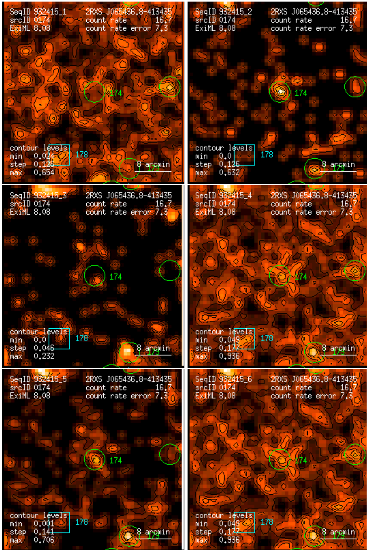
Figure 174: RASS 932415: detection 0174: band rate images, Gaussian filter: (1) PSPC channels 11 – 41, (2) 52 – 90, (3) 91 – 201, (4) 11 – 235, (5) 52 – 201, (6) 11 – 201. Broad band rates in counts/ks. Band rate contour levels in counts/ks/arcmin 2 .
