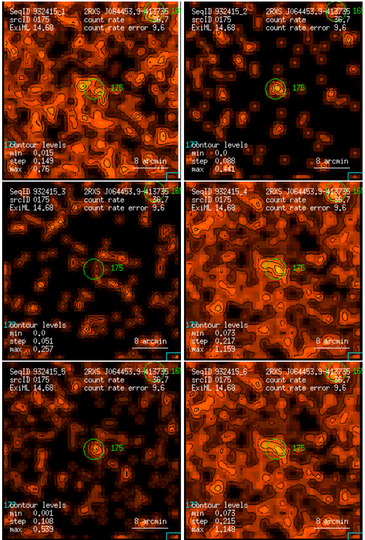
Figure 175: RASS 932415: detection 0175: band rate images, Gaussian filter: (1) PSPC channels 11 – 41, (2) 52 – 90, (3) 91 – 201, (4) 11 – 235, (5) 52 – 201, (6) 11 – 201. Broad band rates in counts/ks. Band rate contour levels in counts/ks/arcmin 2 .
