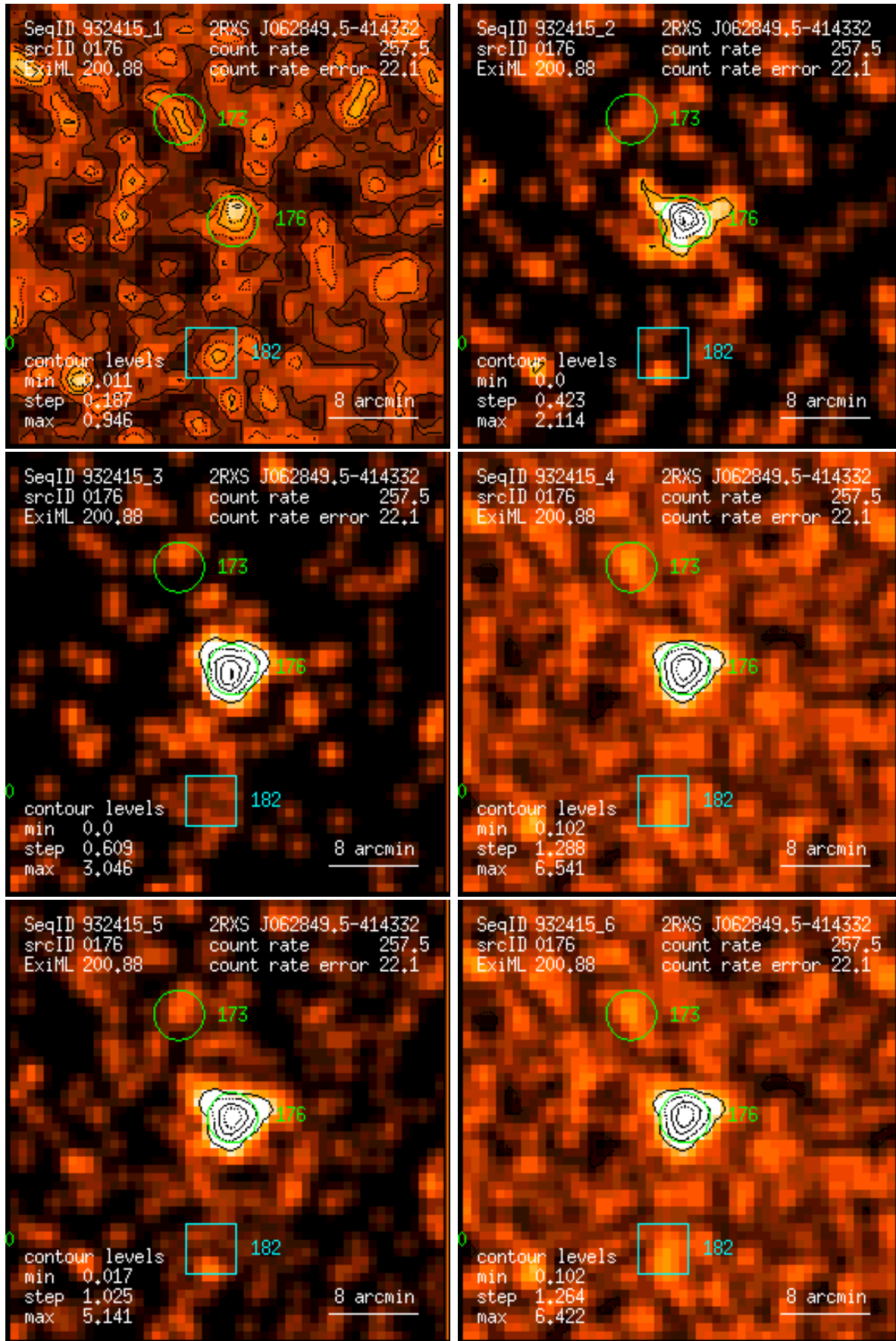
Figure 176: RASS 932415: detection 0176: band rate images, Gaussian filter: (1) PSPC channels 11 – 41, (2) 52 – 90, (3) 91 – 201, (4) 11 – 235, (5) 52 – 201, (6) 11 – 201. Broad band rates in counts/ks. Band rate contour levels in counts/ks/arcmin 2 .
