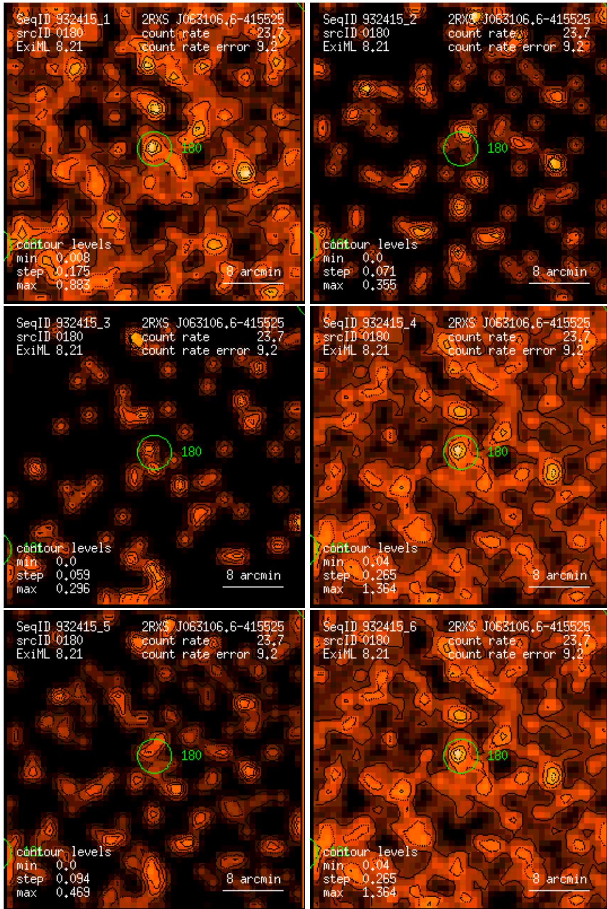
Figure 180: RASS 932415: detection 0180: band rate images, Gaussian filter: (1) PSPC channels 11 – 41, (2) 52 – 90, (3) 91 – 201, (4) 11 – 235, (5) 52 – 201, (6) 11 – 201. Broad band rates in counts/ks. Band rate contour levels in counts/ks/arcmin 2 .
