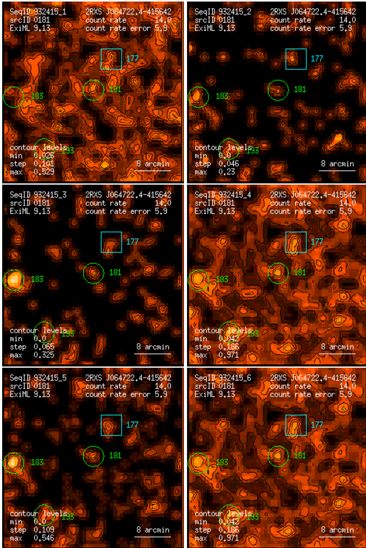
Figure 181: RASS 932415: detection 0181: band rate images, Gaussian filter: (1) PSPC channels 11 – 41, (2) 52 – 90, (3) 91 – 201, (4) 11 – 235, (5) 52 – 201, (6) 11 – 201. Broad band rates in counts/ks. Band rate contour levels in counts/ks/arcmin 2 .
