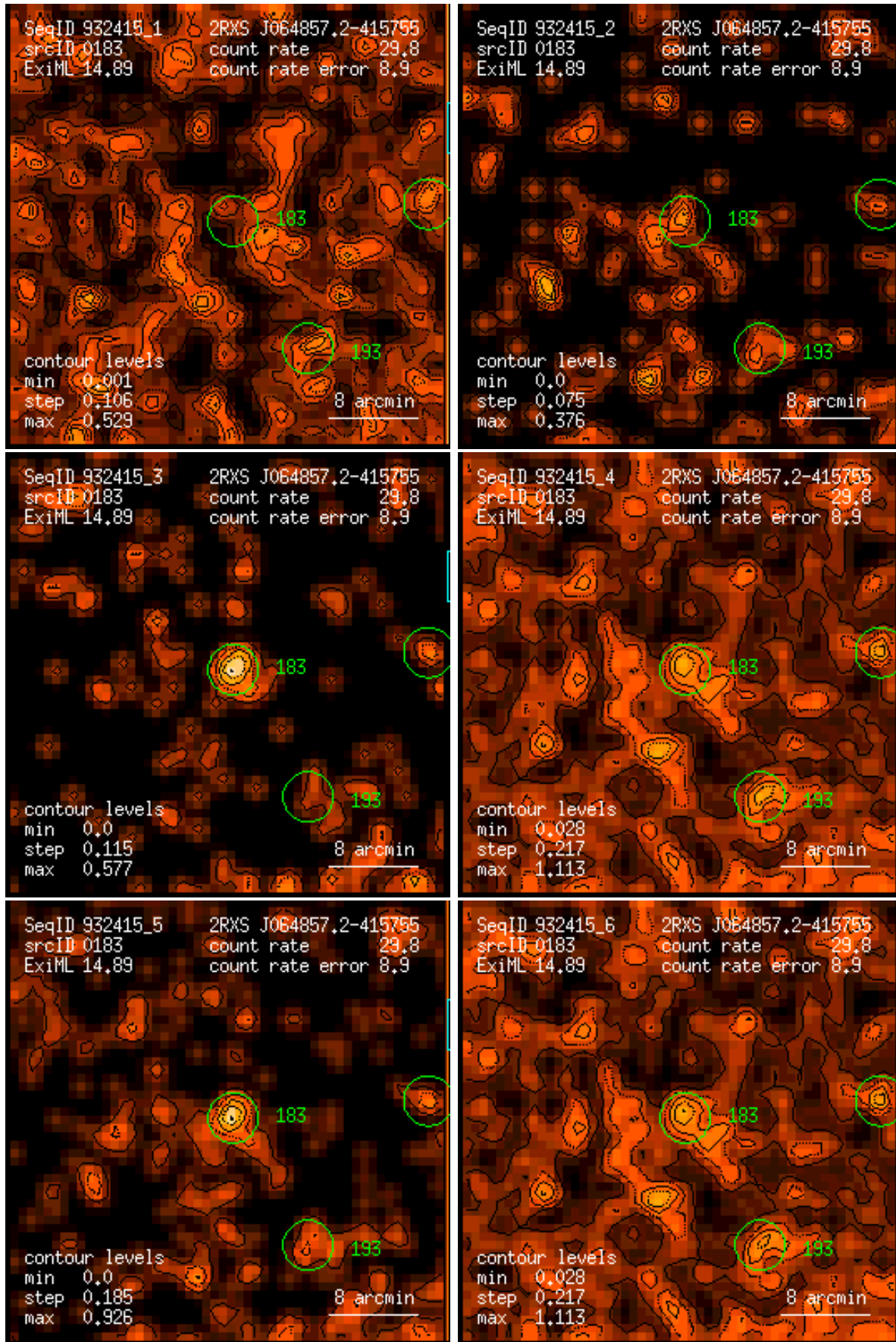
Figure 183: RASS 932415: detection 0183: band rate images, Gaussian filter: (1) PSPC channels 11 – 41, (2) 52 – 90, (3) 91 – 201, (4) 11 – 235, (5) 52 – 201, (6) 11 – 201. Broad band rates in counts/ks. Band rate contour levels in counts/ks/arcmin 2 .
