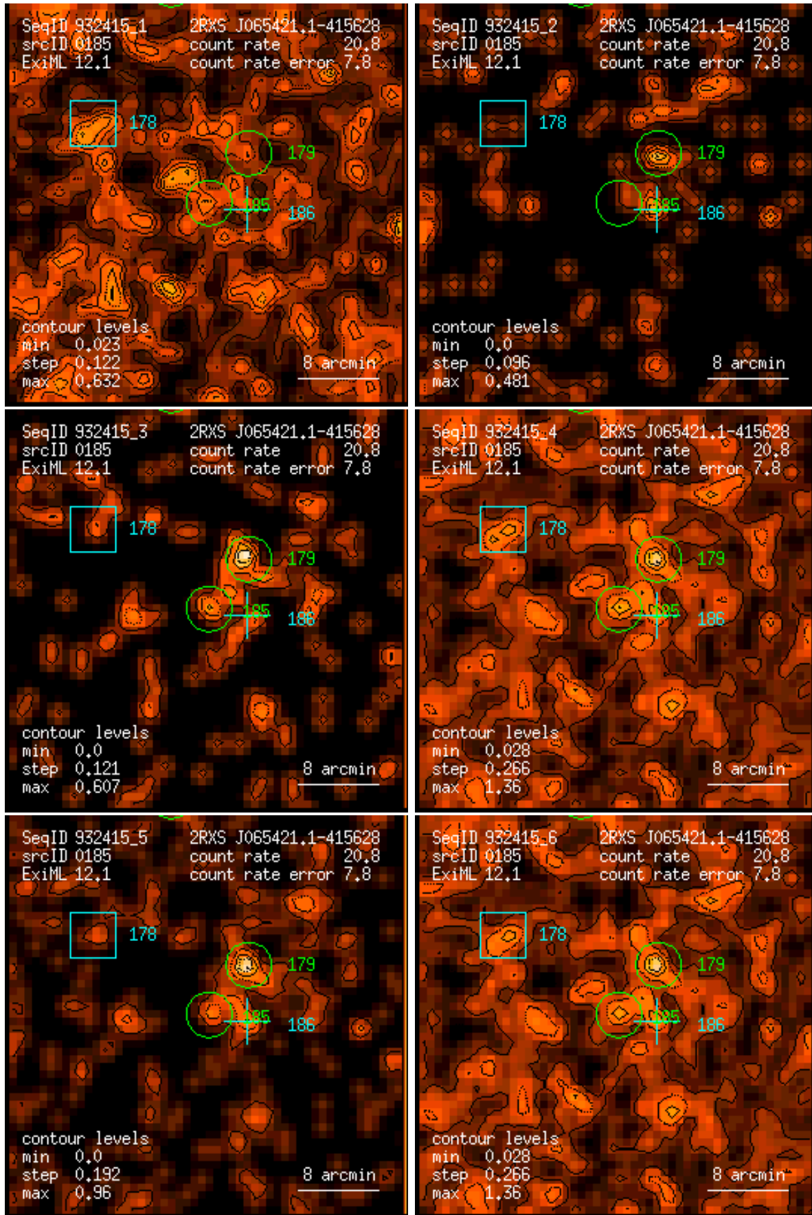
Figure 185: RASS 932415: detection 0185: band rate images, Gaussian filter: (1) PSPC channels 11 – 41, (2) 52 – 90, (3) 91 – 201, (4) 11 – 235, (5) 52 – 201, (6) 11 – 201. Broad band rates in counts/ks. Band rate contour levels in counts/ks/arcmin 2 .
