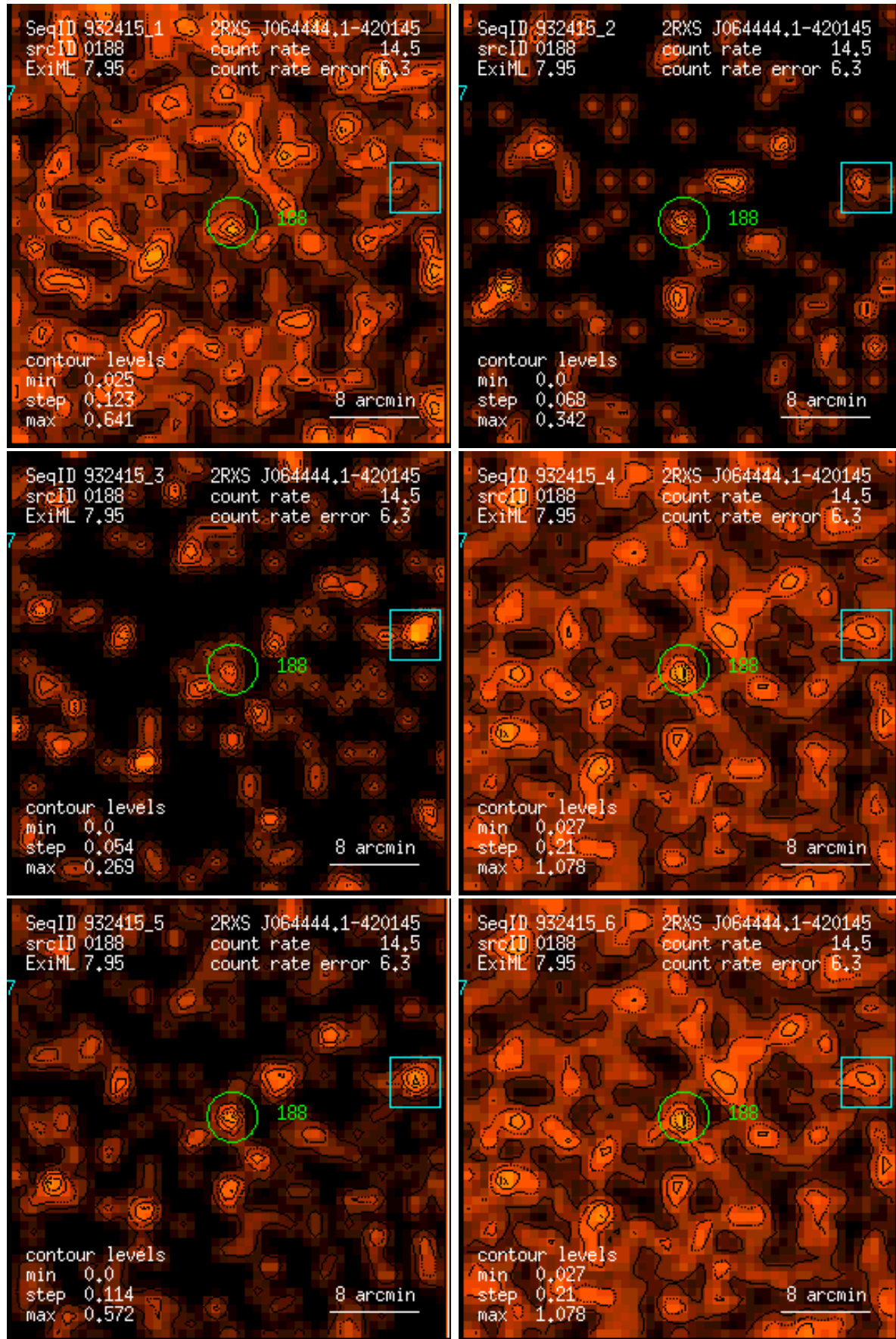
Figure 188: RASS 932415: detection 0188: band rate images, Gaussian filter: (1) PSPC channels 11 – 41, (2) 52 – 90, (3) 91 – 201, (4) 11 – 235, (5) 52 – 201, (6) 11 – 201. Broad band rates in counts/ks. Band rate contour levels in counts/ks/arcmin 2 .
