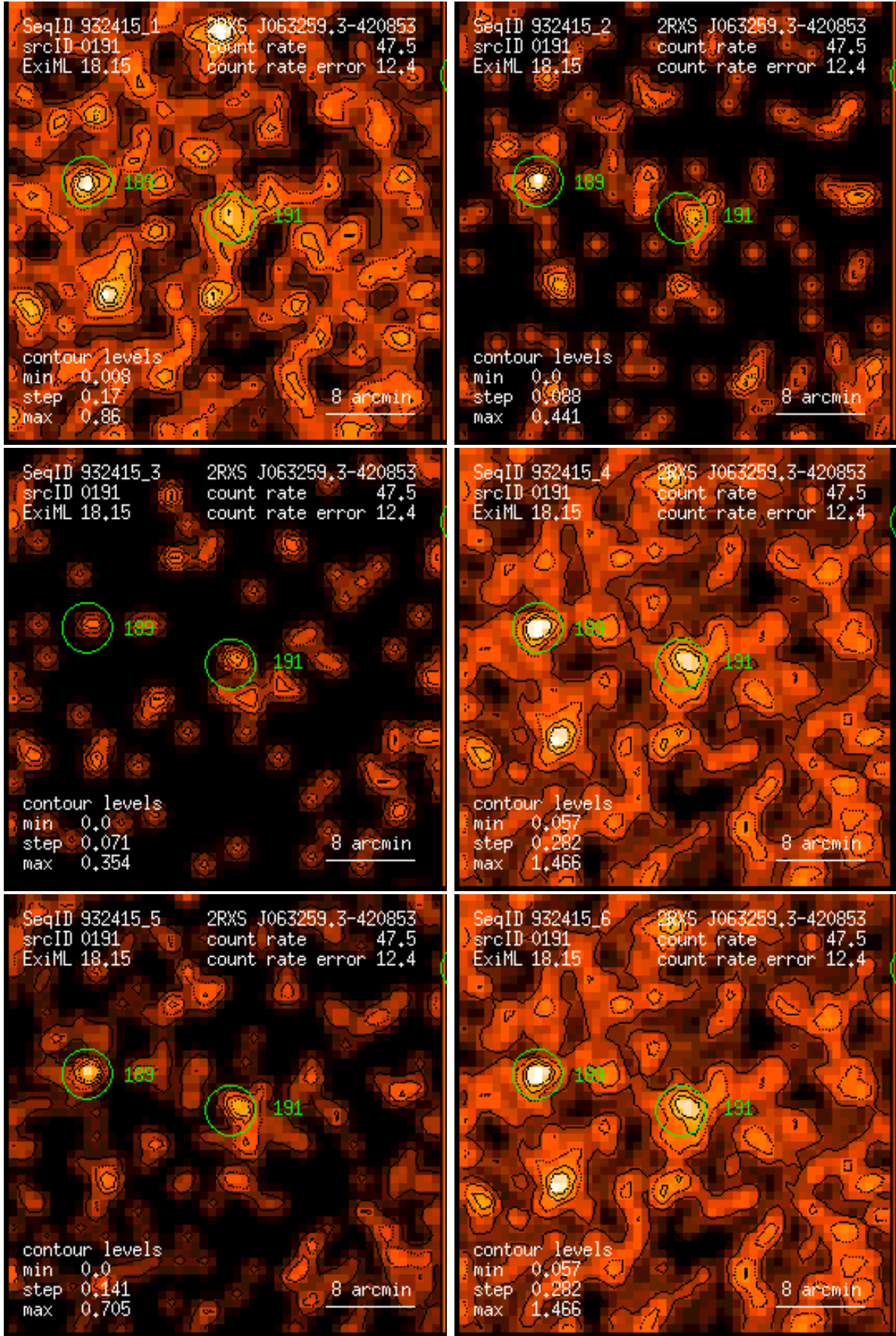
Figure 191: RASS 932415: detection 0191: band rate images, Gaussian filter: (1) PSPC channels 11 – 41, (2) 52 – 90, (3) 91 – 201, (4) 11 – 235, (5) 52 – 201, (6) 11 – 201. Broad band rates in counts/ks. Band rate contour levels in counts/ks/arcmin 2 .
