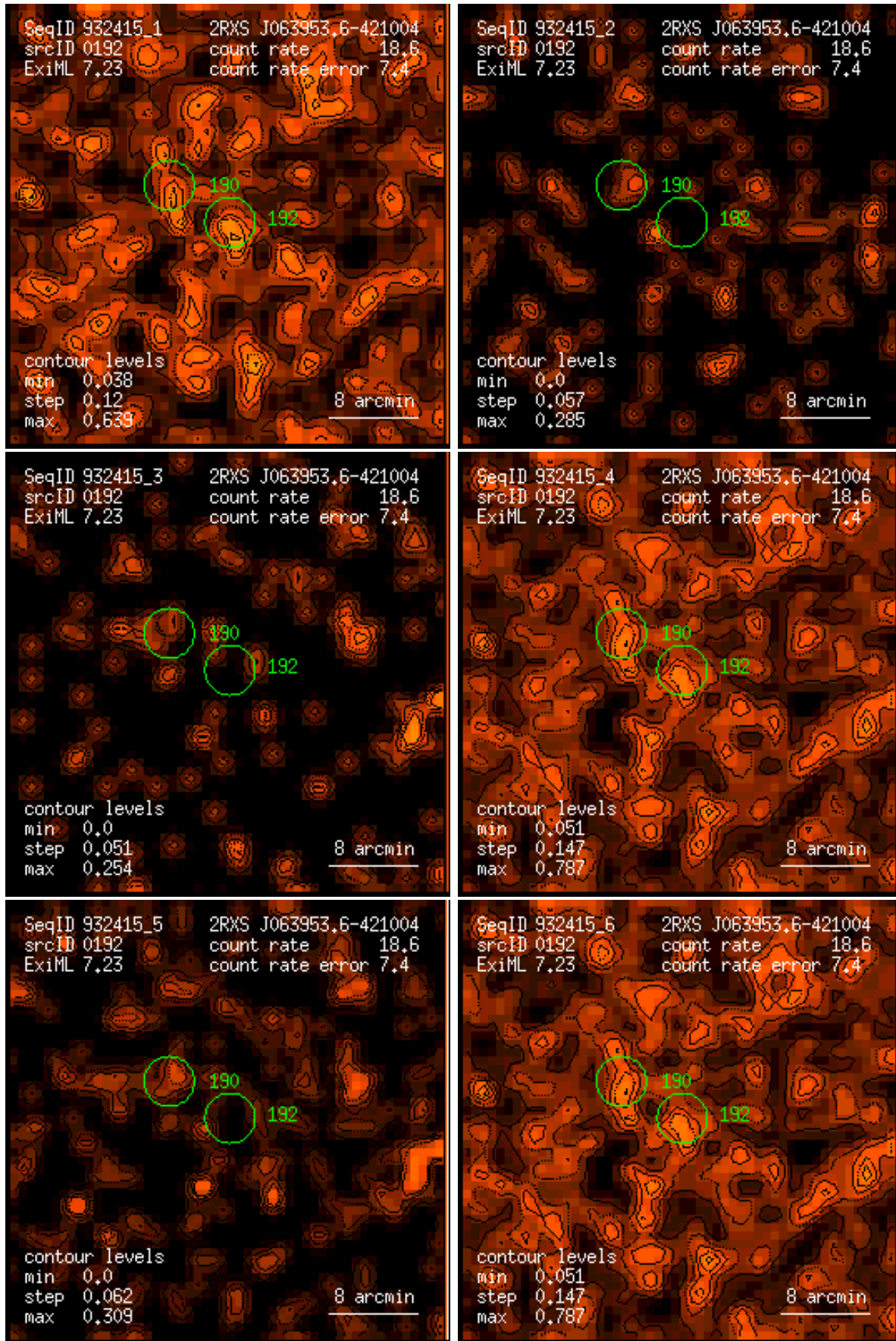
Figure 192: RASS 932415: detection 0192: band rate images, Gaussian filter: (1) PSPC channels 11 – 41, (2) 52 – 90, (3) 91 – 201, (4) 11 – 235, (5) 52 – 201, (6) 11 – 201. Broad band rates in counts/ks. Band rate contour levels in counts/ks/arcmin 2 .
