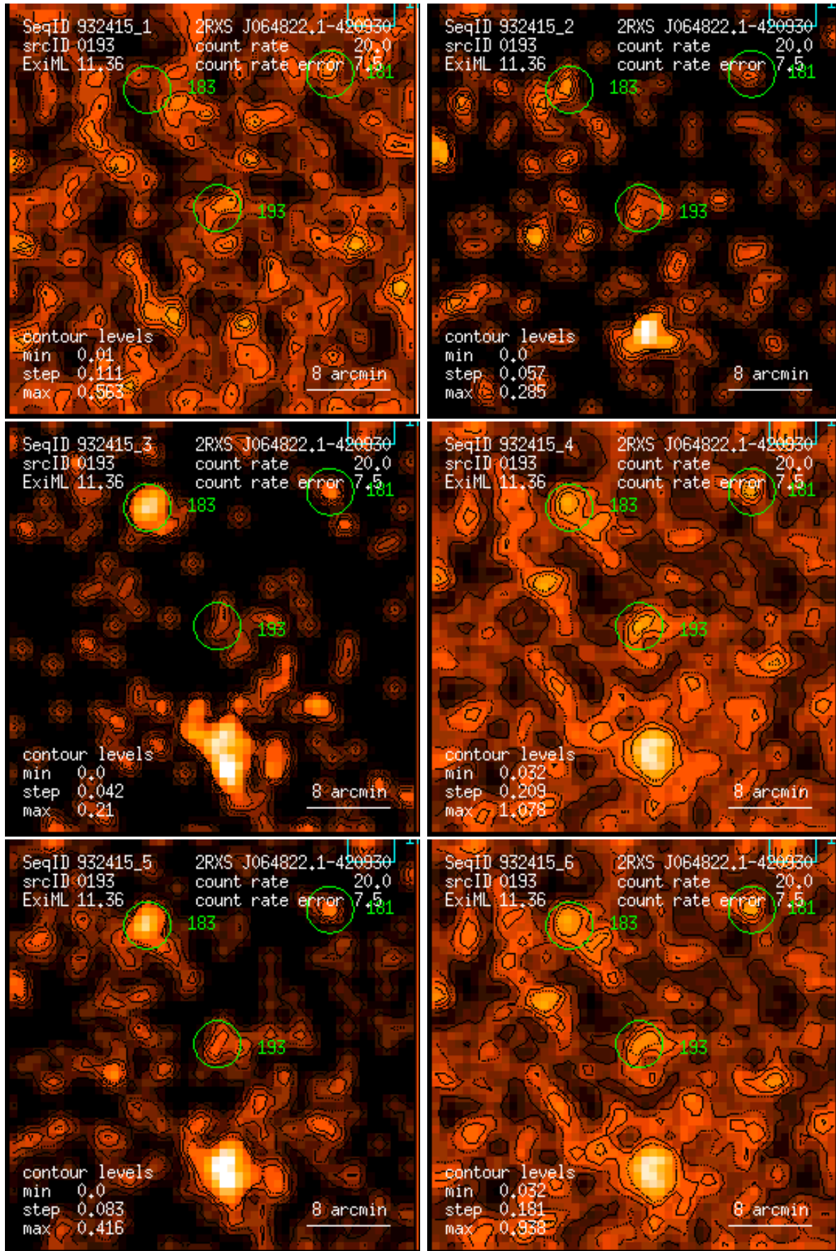
Figure 193: RASS 932415: detection 0193: band rate images, Gaussian filter: (1) PSPC channels 11 – 41, (2) 52 – 90, (3) 91 – 201, (4) 11 – 235, (5) 52 – 201, (6) 11 – 201. Broad band rates in counts/ks. Band rate contour levels in counts/ks/arcmin 2 .
