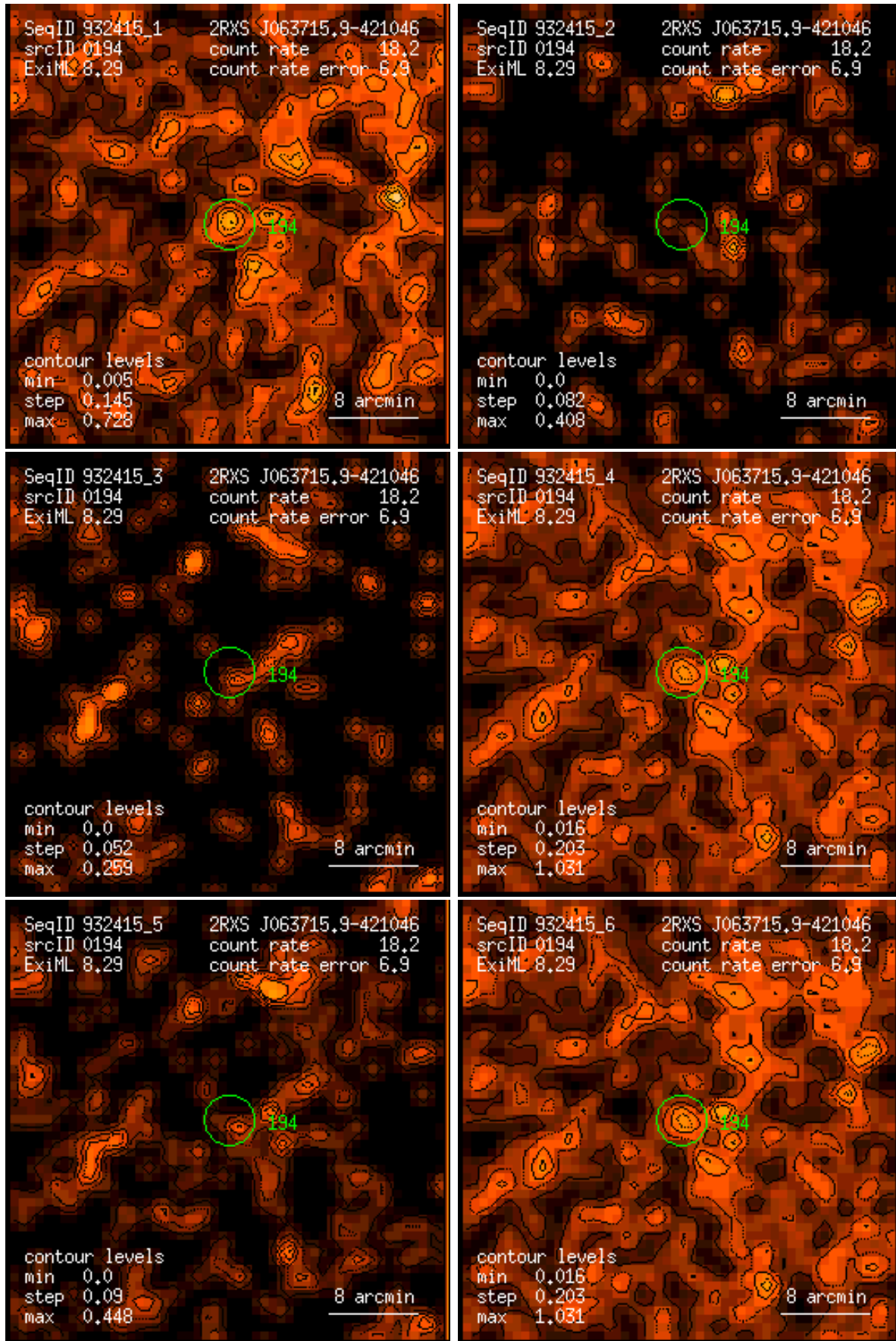
Figure 194: RASS 932415: detection 0194: band rate images, Gaussian filter: (1) PSPC channels 11 – 41, (2) 52 – 90, (3) 91 – 201, (4) 11 – 235, (5) 52 – 201, (6) 11 – 201. Broad band rates in counts/ks. Band rate contour levels in counts/ks/arcmin 2 .
