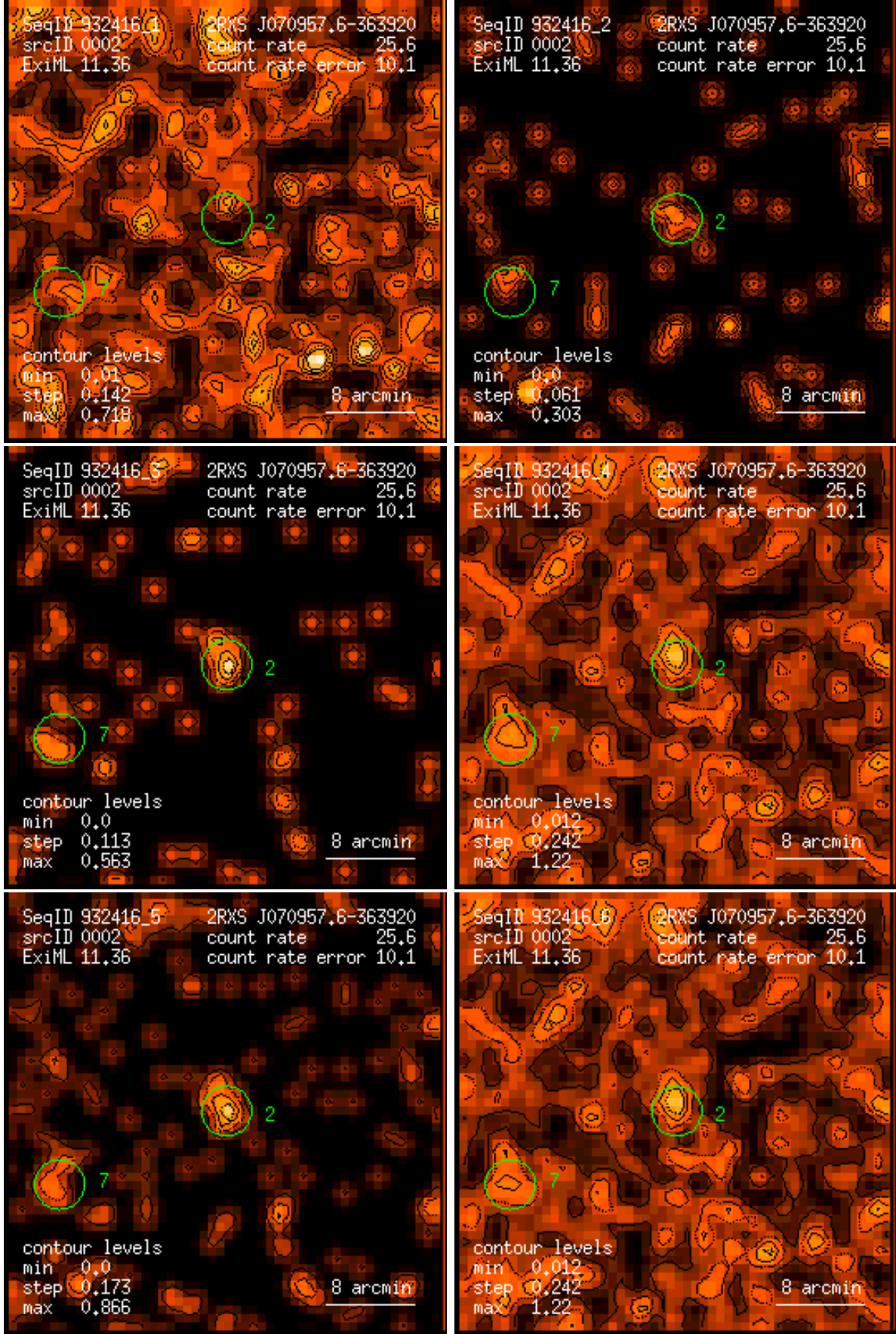
Figure 2: RASS 932416: detection 0002: band rate images, Gaussian filter: (1) PSPC channels 11 – 41, (2) 52 – 90, (3) 91 – 201, (4) 11 – 235, (5) 52 – 201, (6) 11 – 201. Broad band rates in counts/ks. Band rate contour levels in counts/ks/arcmin 2 .
