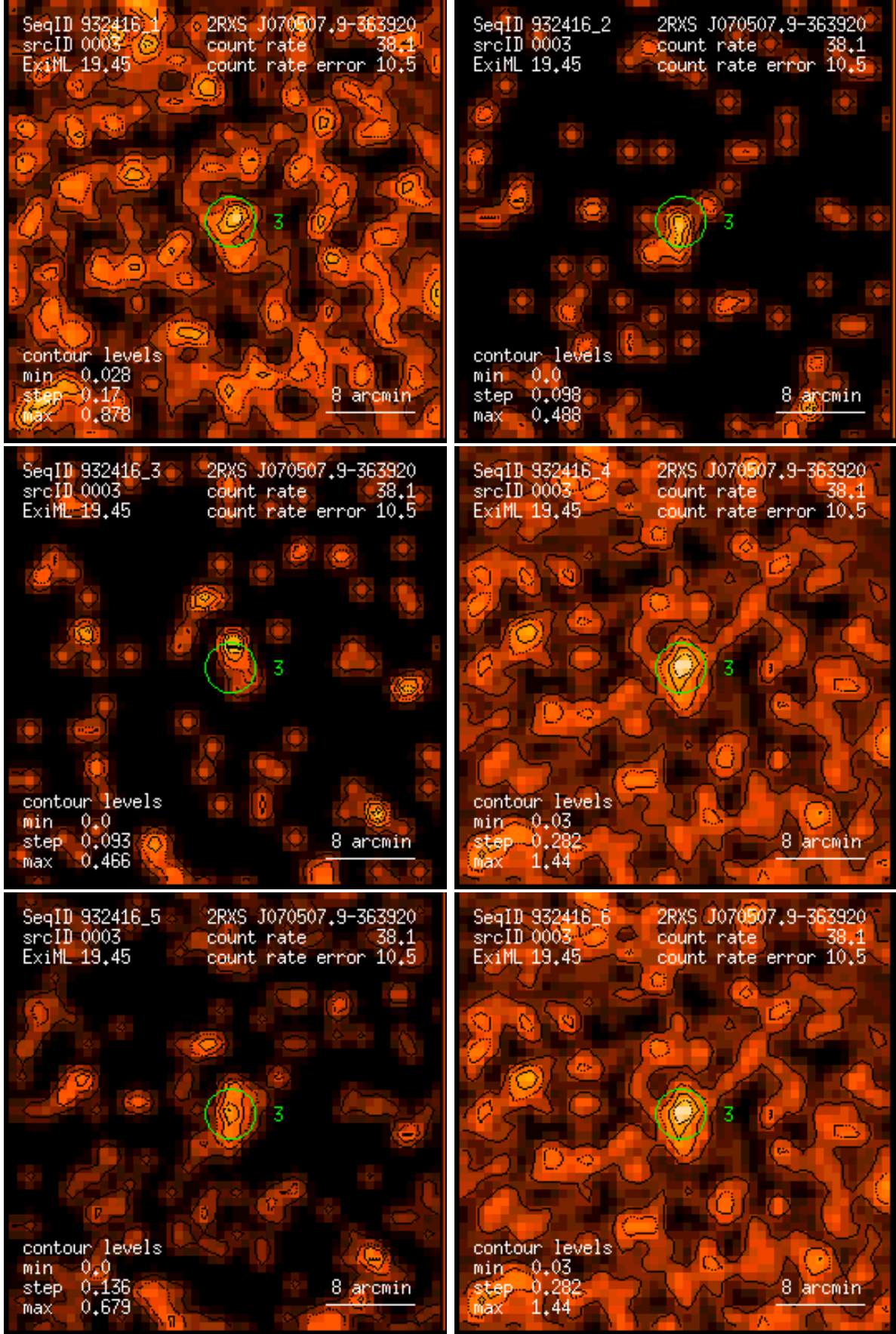
Figure 3: RASS 932416: detection 0003: band rate images, Gaussian filter: (1) PSPC channels 11 – 41, (2) 52 – 90, (3) 91 – 201, (4) 11 – 235, (5) 52 – 201, (6) 11 – 201. Broad band rates in counts/ks. Band rate contour levels in counts/ks/arcmin 2 .
