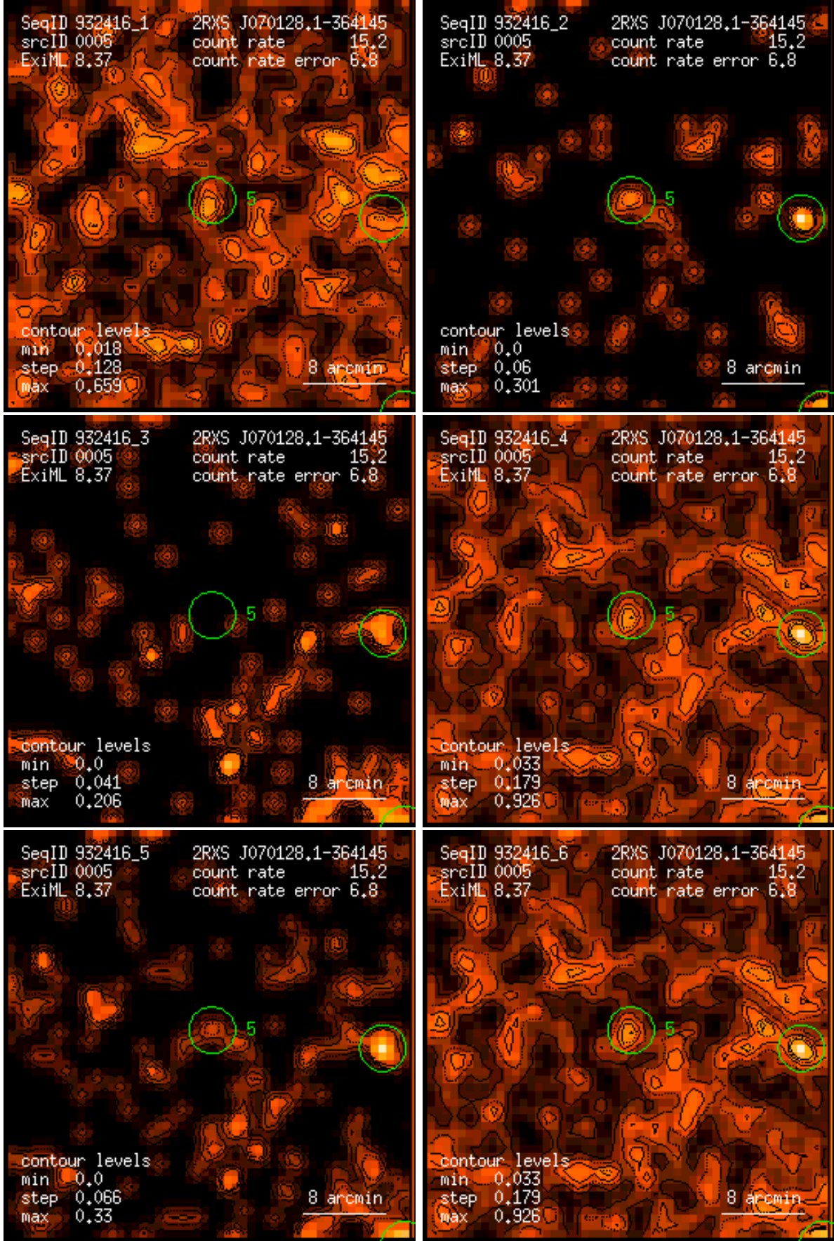
Figure 5: RASS 932416: detection 0005: band rate images, Gaussian filter: (1) PSPC channels 11 – 41, (2) 52 – 90, (3) 91 – 201, (4) 11 – 235, (5) 52 – 201, (6) 11 – 201. Broad band rates in counts/ks. Band rate contour levels in counts/ks/arcmin 2 .
