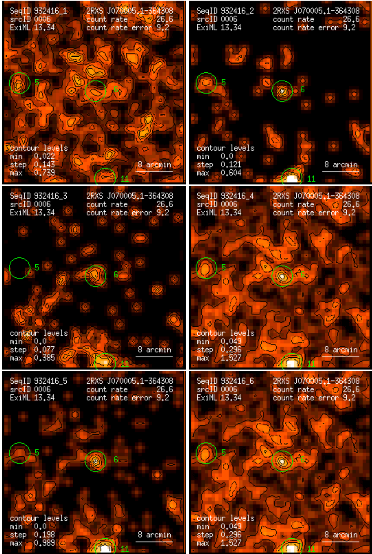
Figure 6: RASS 932416: detection 0006: band rate images, Gaussian filter: (1) PSPC channels 11 – 41, (2) 52 – 90, (3) 91 – 201, (4) 11 – 235, (5) 52 – 201, (6) 11 – 201. Broad band rates in counts/ks. Band rate contour levels in counts/ks/arcmin 2 .
