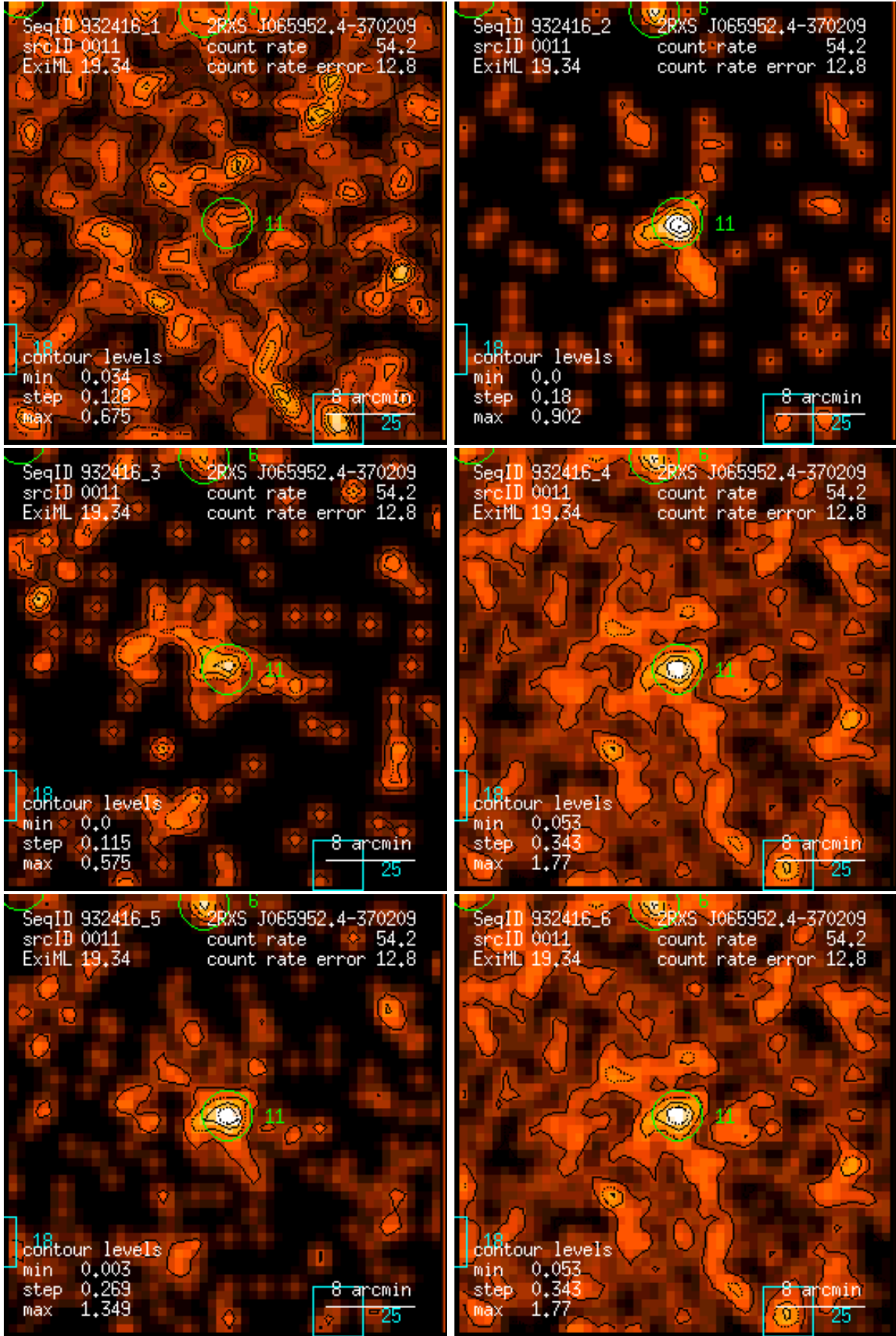
Figure 11: RASS 932416: detection 0011: band rate images, Gaussian filter: (1) PSPC channels 11 – 41, (2) 52 – 90, (3) 91 – 201, (4) 11 – 235, (5) 52 – 201, (6) 11 – 201. Broad band rates in counts/ks. Band rate contour levels in counts/ks/arcmin 2 .
