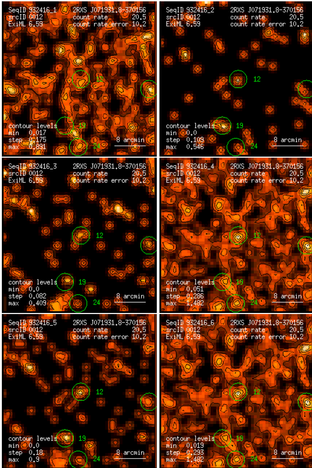
Figure 12: RASS 932416: detection 0012: band rate images, Gaussian filter: (1) PSPC channels 11 – 41, (2) 52 – 90, (3) 91 – 201, (4) 11 – 235, (5) 52 – 201, (6) 11 – 201. Broad band rates in counts/ks. Band rate contour levels in counts/ks/arcmin 2 .
