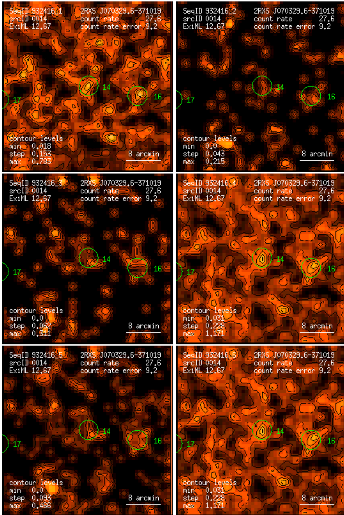
Figure 14: RASS 932416: detection 0014: band rate images, Gaussian filter: (1) PSPC channels 11 – 41, (2) 52 – 90, (3) 91 – 201, (4) 11 – 235, (5) 52 – 201, (6) 11 – 201. Broad band rates in counts/ks. Band rate contour levels in counts/ks/arcmin 2 .
