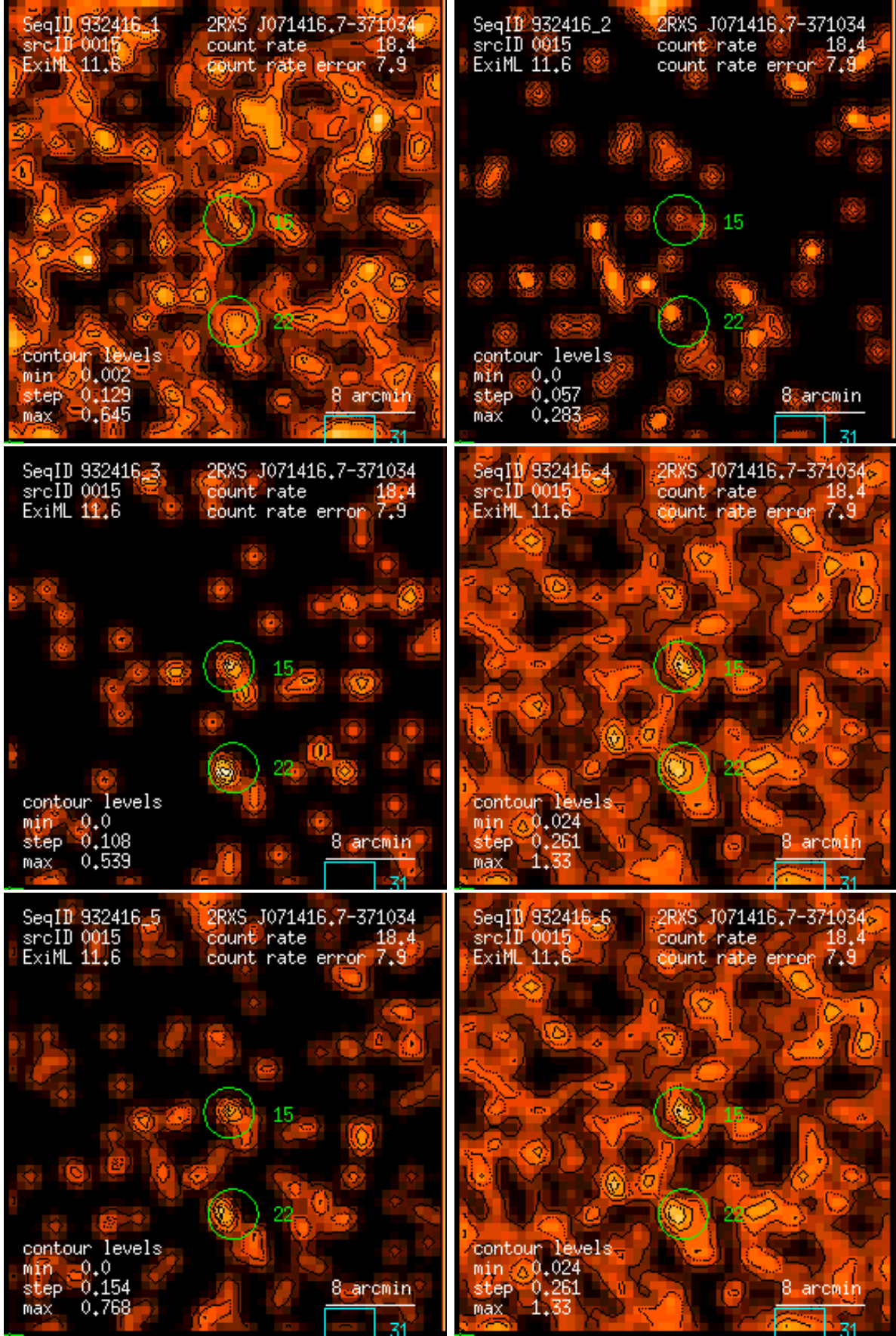
Figure 15: RASS 932416: detection 0015: band rate images, Gaussian filter: (1) PSPC channels 11 – 41, (2) 52 – 90, (3) 91 – 201, (4) 11 – 235, (5) 52 – 201, (6) 11 – 201. Broad band rates in counts/ks. Band rate contour levels in counts/ks/arcmin 2 .
