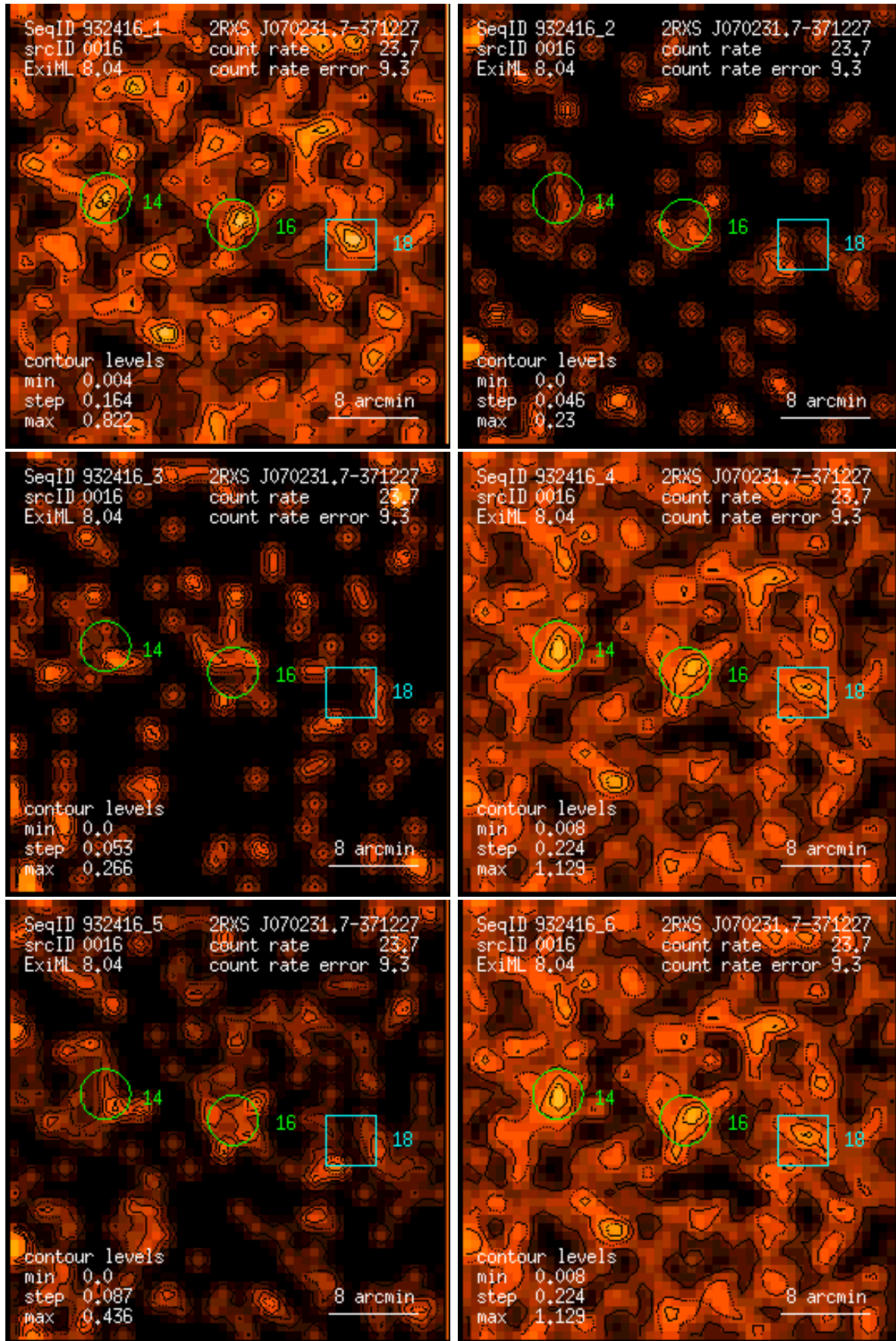
Figure 16: RASS 932416: detection 0016: band rate images, Gaussian filter: (1) PSPC channels 11 – 41, (2) 52 – 90, (3) 91 – 201, (4) 11 – 235, (5) 52 – 201, (6) 11 – 201. Broad band rates in counts/ks. Band rate contour levels in counts/ks/arcmin 2 .
