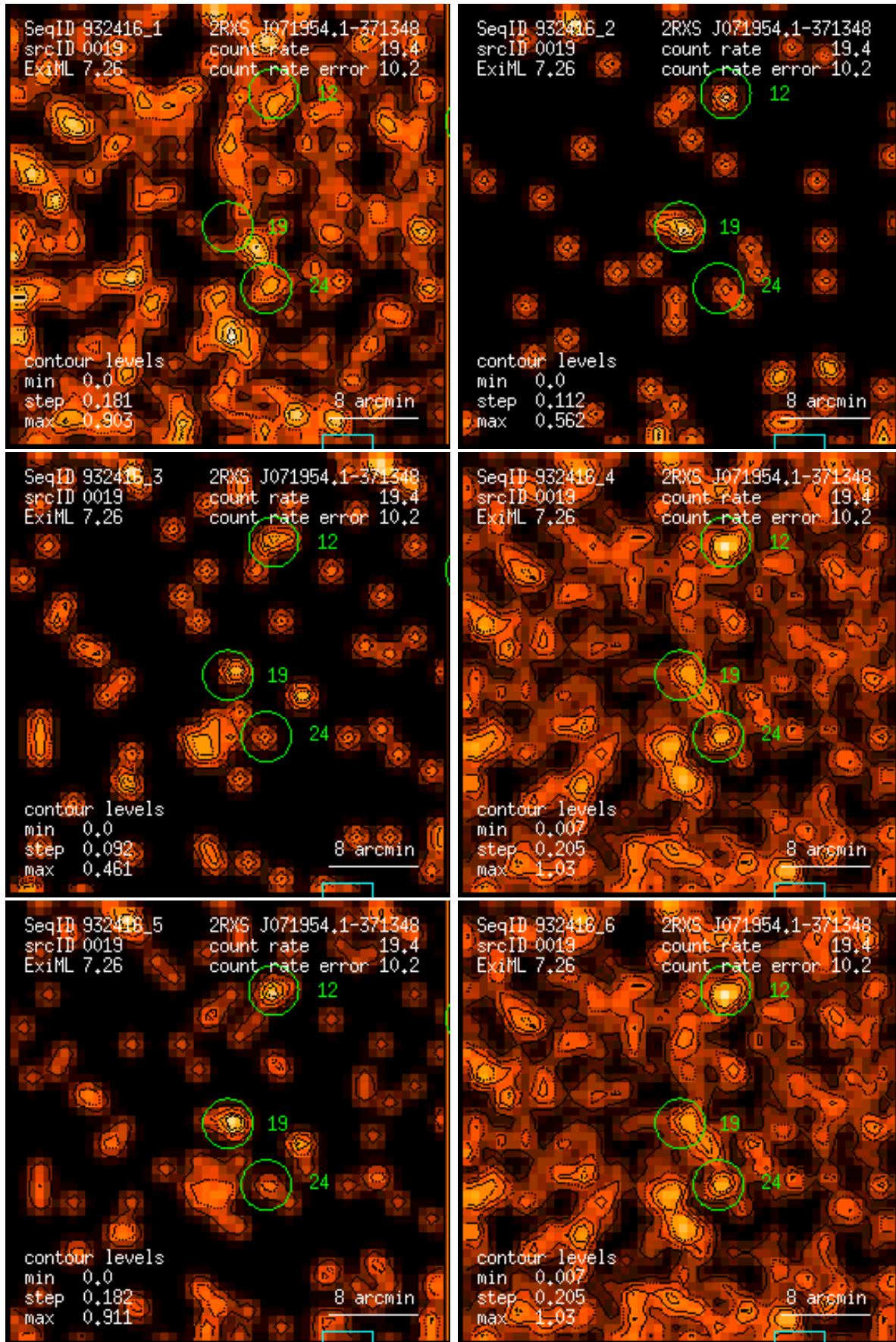
Figure 19: RASS 932416: detection 0019: band rate images, Gaussian filter: (1) PSPC channels 11 – 41, (2) 52 – 90, (3) 91 – 201, (4) 11 – 235, (5) 52 – 201, (6) 11 – 201. Broad band rates in counts/ks. Band rate contour levels in counts/ks/arcmin 2 .
