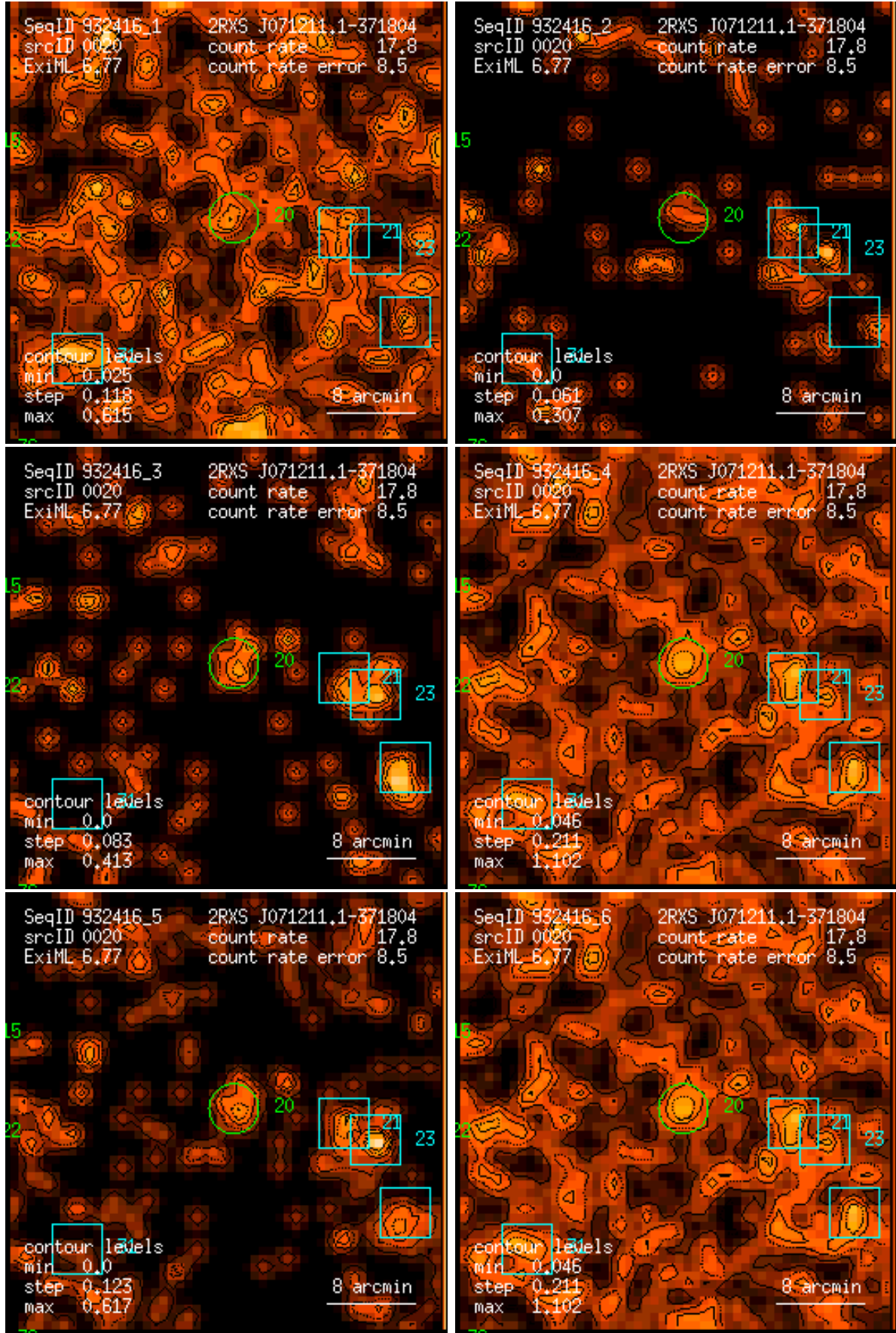
Figure 20: RASS 932416: detection 0020: band rate images, Gaussian filter: (1) PSPC channels 11 – 41, (2) 52 – 90, (3) 91 – 201, (4) 11 – 235, (5) 52 – 201, (6) 11 – 201. Broad band rates in counts/ks. Band rate contour levels in counts/ks/arcmin 2 .
